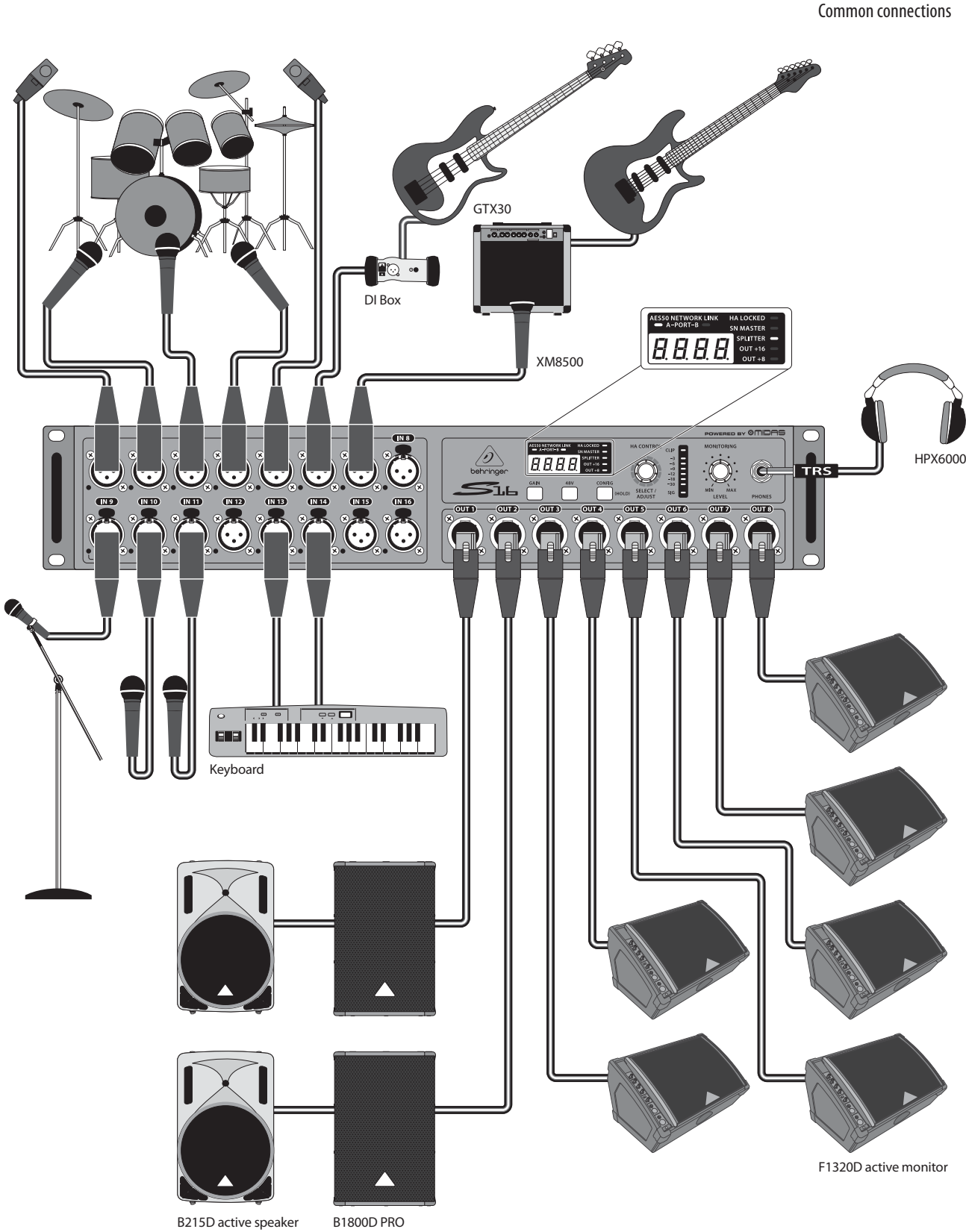
Common connections
