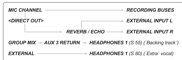
Fig. 14.4: Subgroup-driven auxless headphones mix
