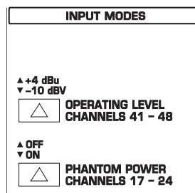
Fig. 7.9: MIX-B operating level switch and phantom power switch
