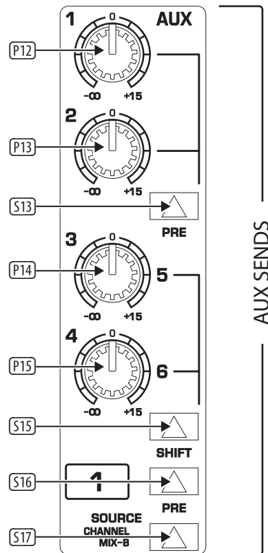
Fig. 3.4: Aux sends
