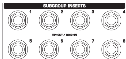
Fig. 7.4: Subgroup inserts
