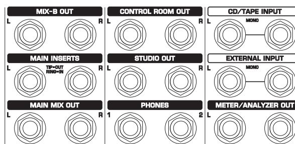
Fig. 7.6: Additional connectors
