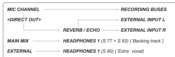
Fig. 14.2: Simple auxless headphones mix
