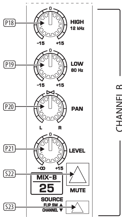
Fig. 3.6: B-channel
