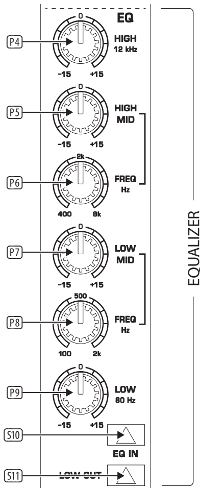
Fig. 3.3: Main equalizer
