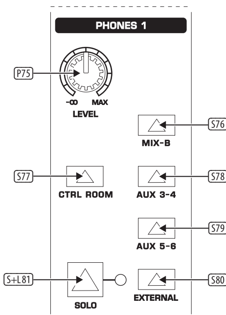
Fig. 6.5: Phones
