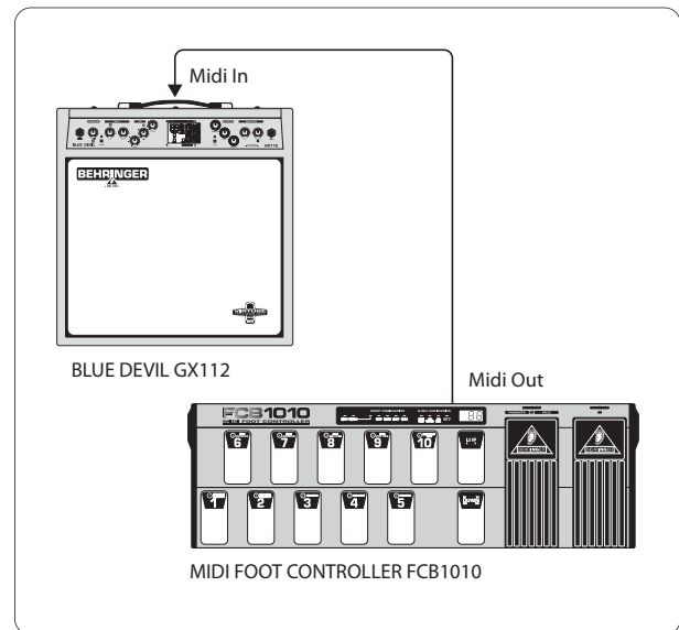
Fig. 3.1: Basic setup with a guitar amp
