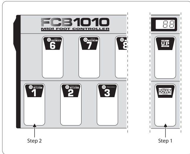
Fig. 2.1: PRESET selection with DIRECT SELECT disabled
