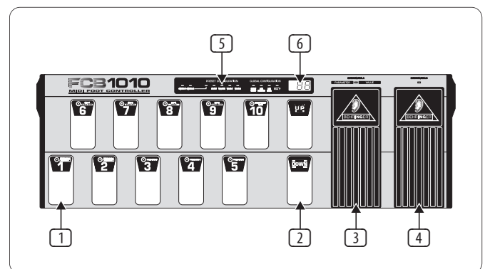
Fig. 1.1: Front panel control elements
