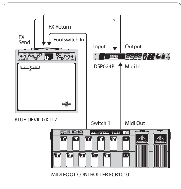
Fig. 3.2: Guitar setup (using the switch function)
