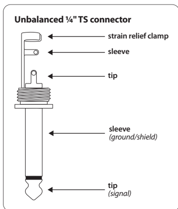
Fig. 4.1: 1/4" TS connector
