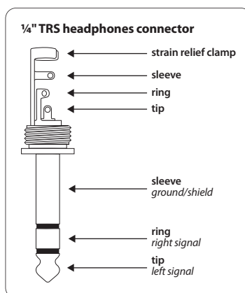
Fig. 4.4: 1/4" TRS connector for headphones operation
