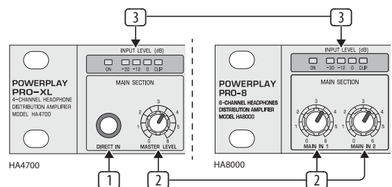
Fig. 2.1: Input section
