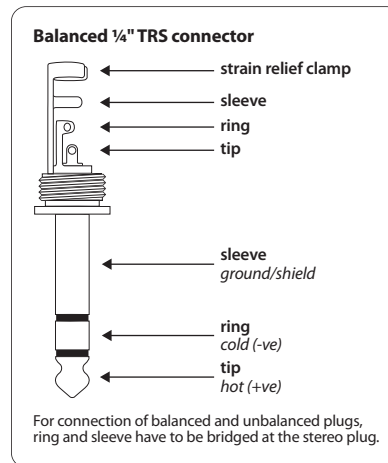
Fig. 5.1: 1/4" TRS connector
