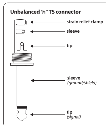
Fig. 5.2: 1/4" TS connector
