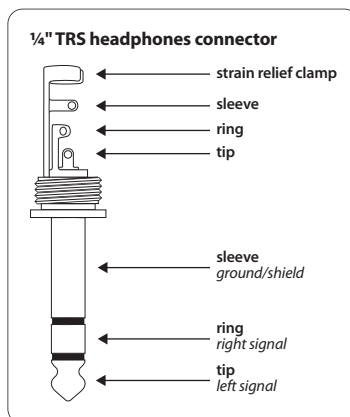
Fig. 4.5: ¼" TRS connector for headphones
