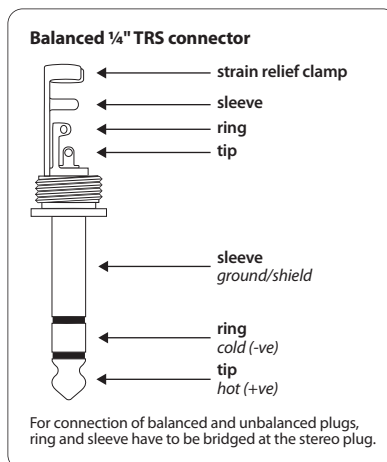
Fig. 4.4: ¼" TRS connector
