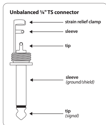
Fig. 4.3: ¼" TS connector
