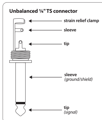
Fig. 4.3: 1/4" TS connector
