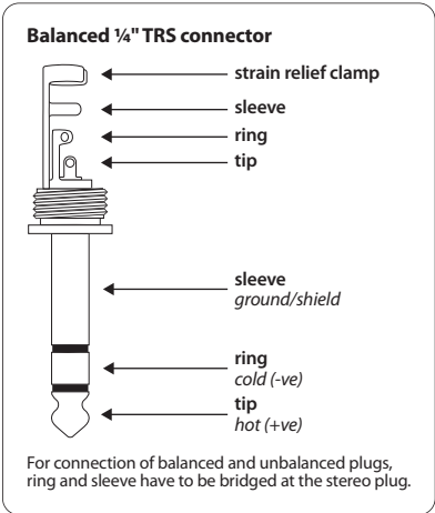
Fig. 4.4: 1/4" TRS connector
