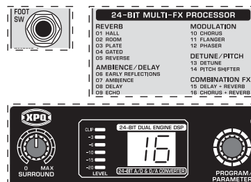
Fig. 3.1: Effects presets overview
