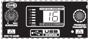
Fig. 3.3: Digital Effects module and XPQ Surround Function control elements
