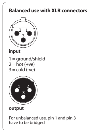
Fig. 4.2: XLR connections
