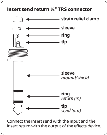
Fig. 4.5: Insert send return 1/4" TRS connector
