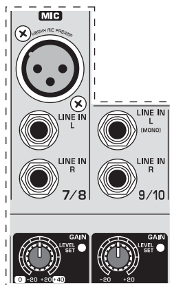
Fig. 2.5: Stereo channel inputs
