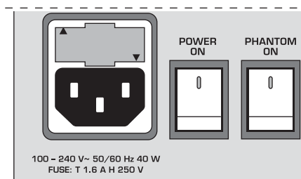
Fig. 2.17: Voltage supply and fuse
