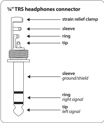
Fig. 4.6: 1/4" TRS connector for headphones
