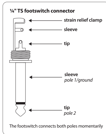
Fig. 4.1: 1/4" TS footswitch connector
