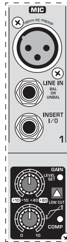
Fig. 2.1: Connectors and controls of mic/line inputs
