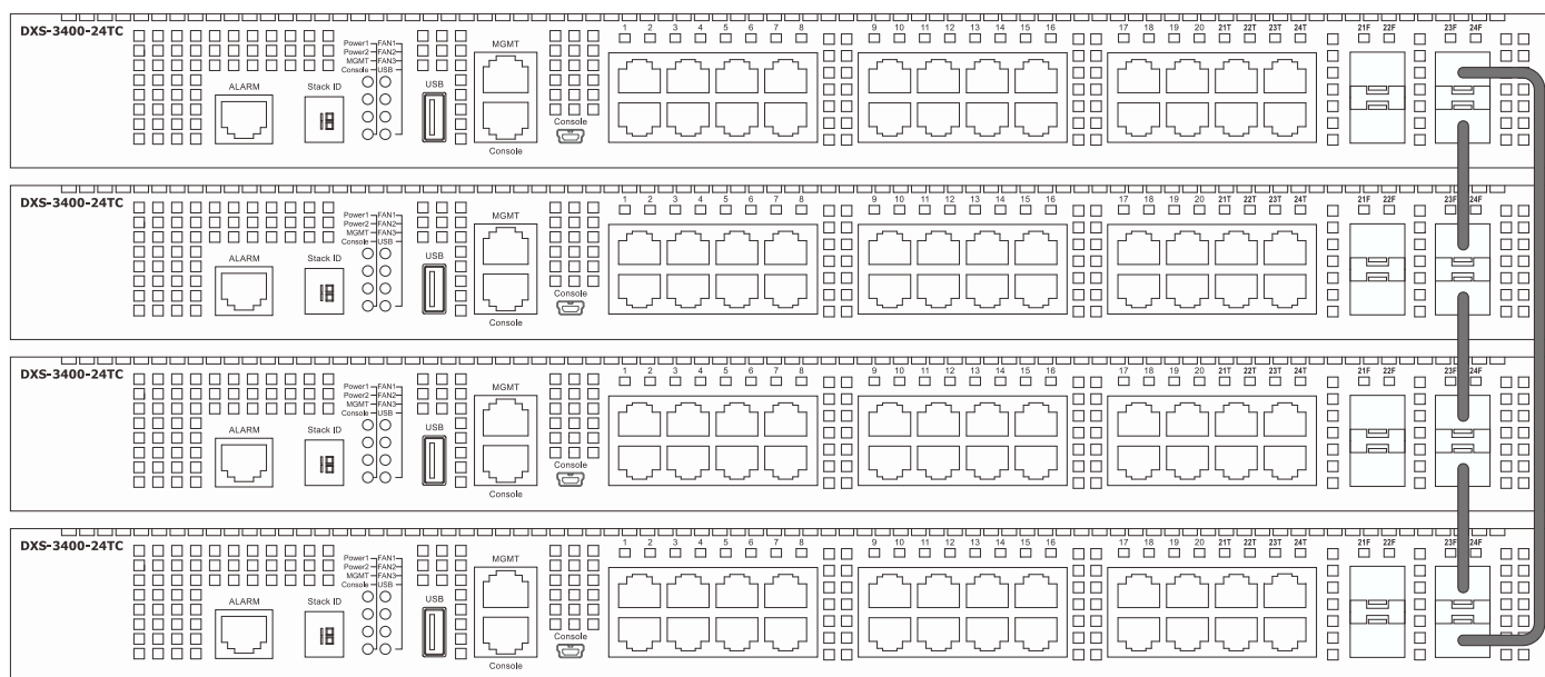
Figure 4-78 Duplex Ring stacking topology (SFP+)
