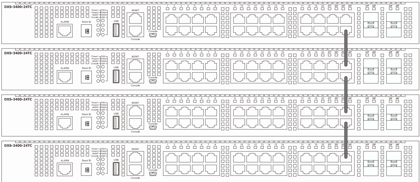
Figure 4-75 Duplex Chain stacking topology (RJ45)
