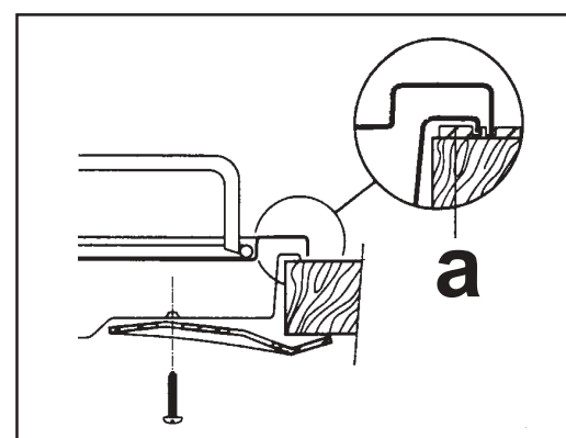
a) Sealing gasket
