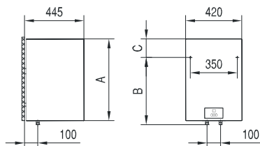
Connection and installation dimensions of the water heater [mm]
