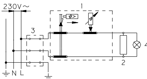
Electric installation
