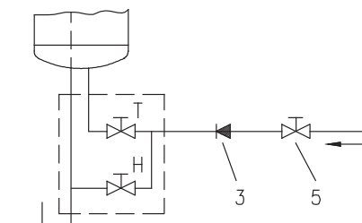
Open (non-pressure) system
