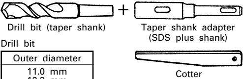
Cotter
