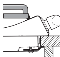
Hooking position for top H=20 mm
