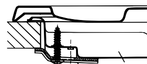
Hooking position for top H=20 mm
