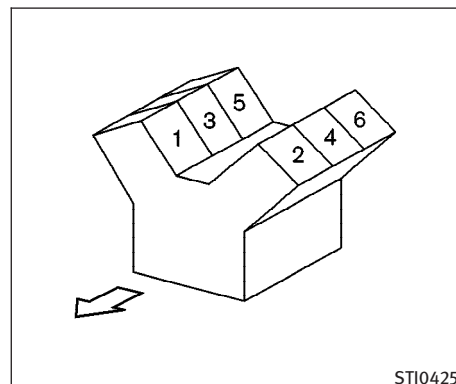
VQ35HR engine
