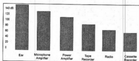
Chart. 1 The dynamic range capabilities of various devices
