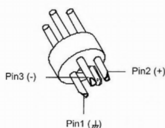
XLR Type Balanced
