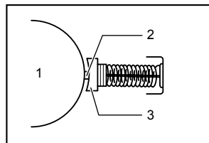
1. Commutator 2. Insulating tip 3. Carbon brush
