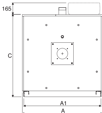
RTQ 297÷467
