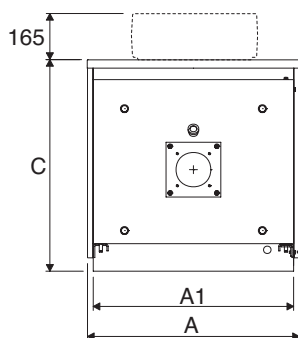
RTQ 297÷467
