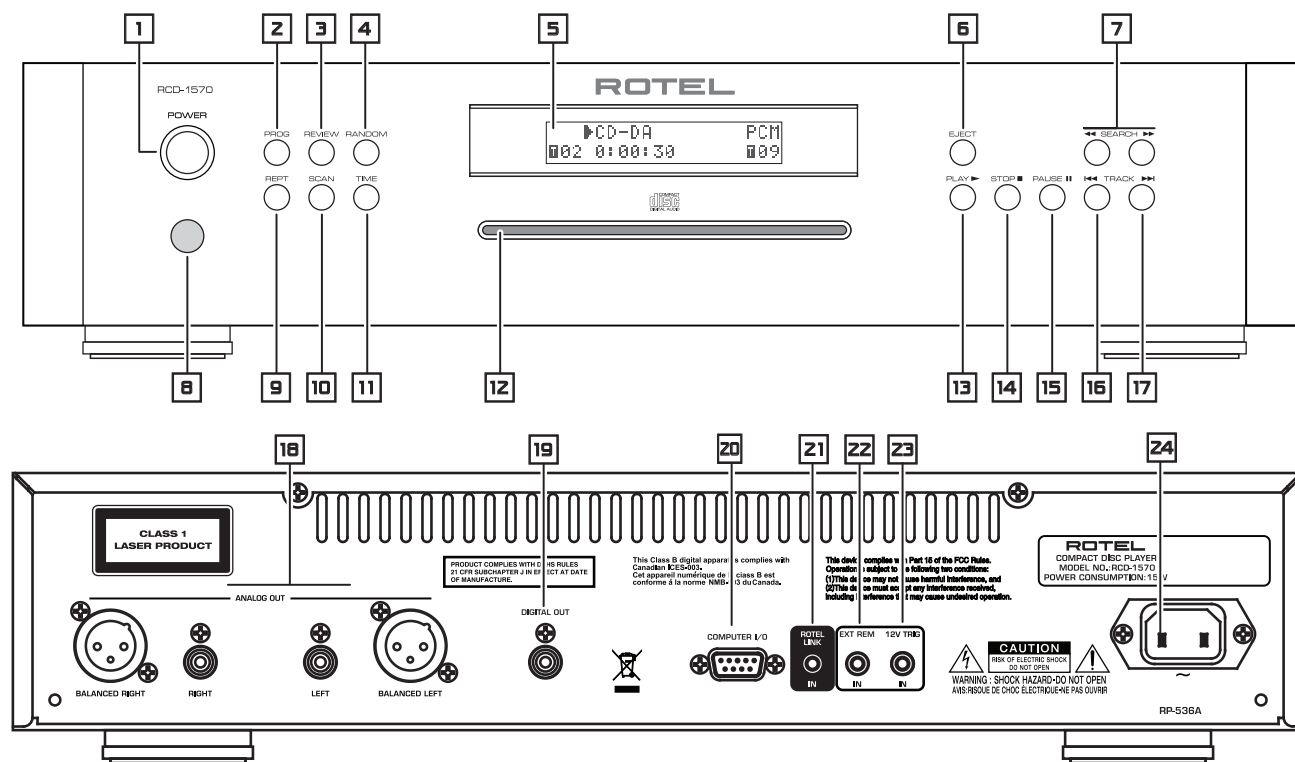
Figure 1: Controls and Connections Commandes et Branchements Bedienelemente und Anschlüsse Controlles y Conexiones
