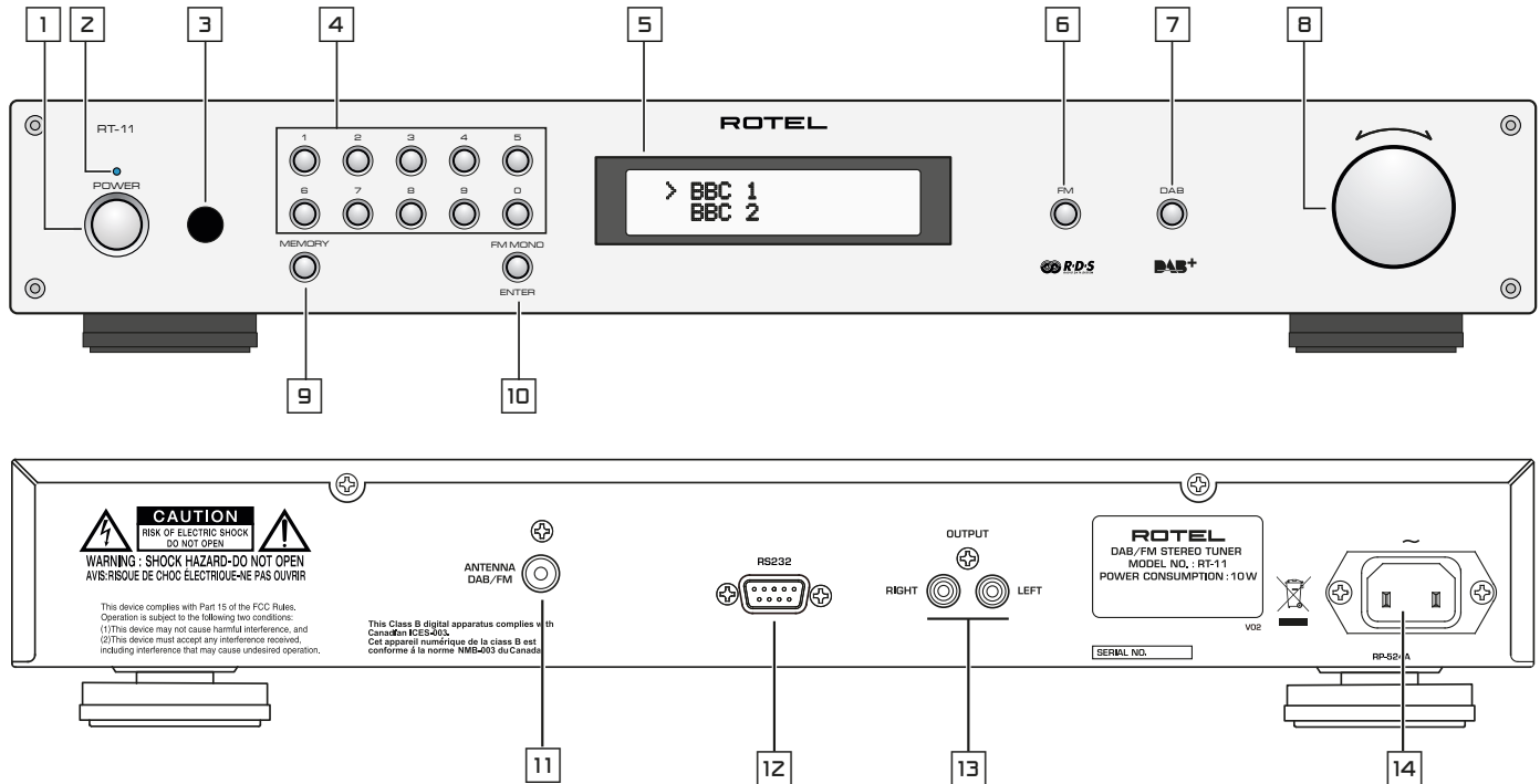
Figure 1: Controls and Connections Commandes et Branchements Bedienelemente und Anschlüsse Controlles y Conexiones
