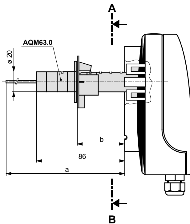
QAF64... with depth-adjustable mounting flange AQM63.0
