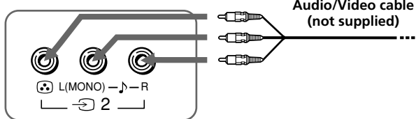
TV front panel
