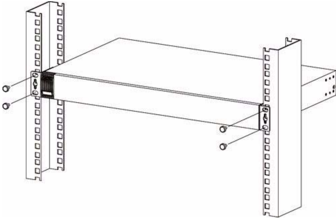
Figure 9 Mounting the Switch on a Rack (ES1100-24)
