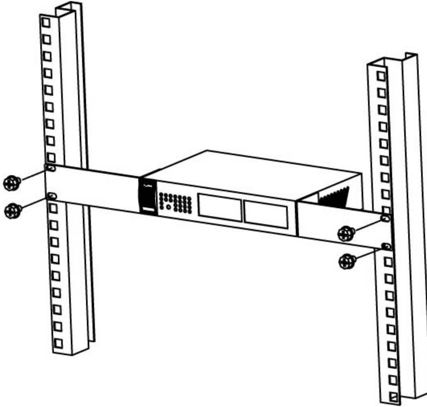
Figure 8 Mounting the Switch on a Rack (ES1100-16/24E)
