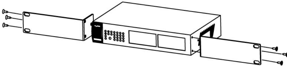
Figure 7 Attaching the Mounting Brackets (ES1100-24)
