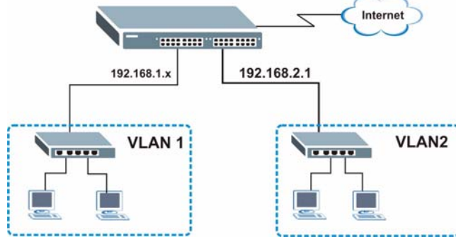
Figure 21 Initial Setup Example: Management IP Address
