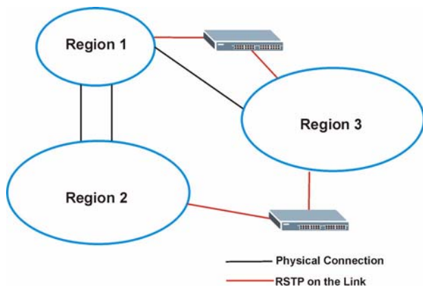
Figure 78 MSTP and Legacy RSTP Network Example
