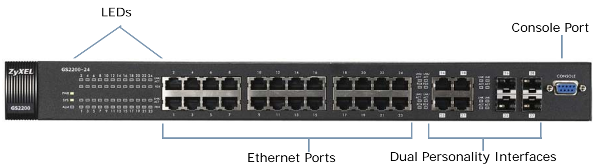
Figure 7 Front Panel (GS200-24)
