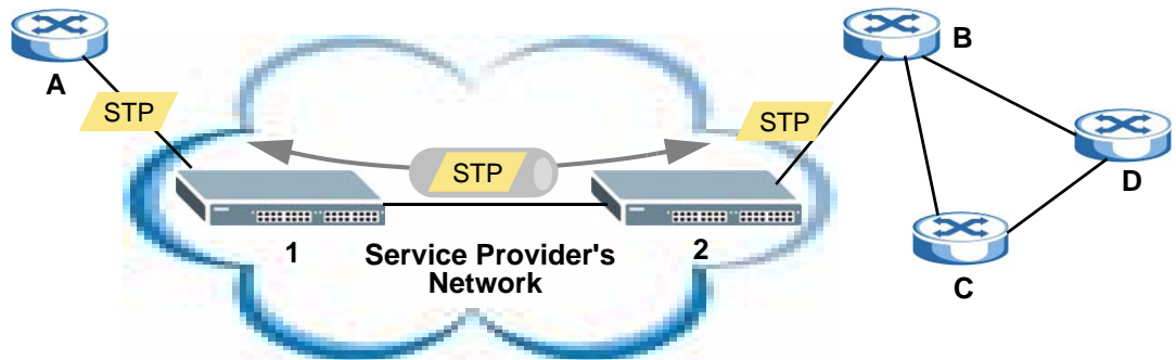
Figure 135 L2PT Network Example
