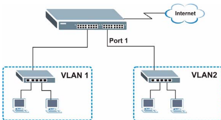
Figure 19 Initial Setup Network Example: VLAN
