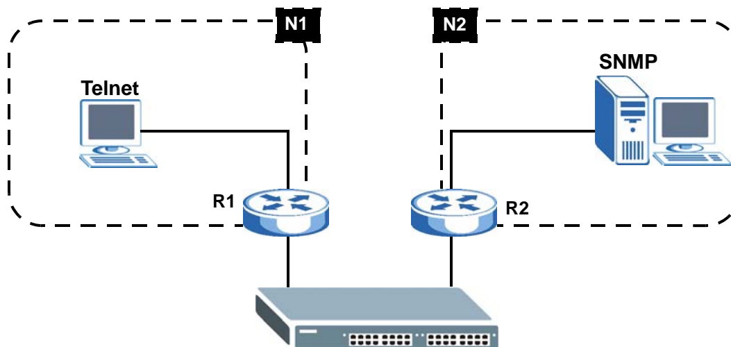
Figure 137 Static Routing Overview
