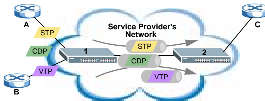
Figure 134 Layer 2 Protocol Tunneling Network Scenario
