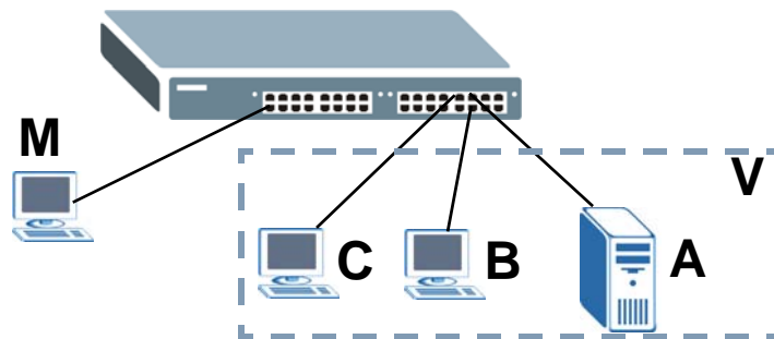
Figure 22 Tutorial: DHCP Snooping Tutorial Overview
