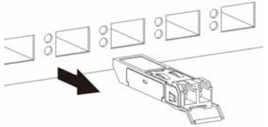
Figure 13 Transceiver Removal Example
