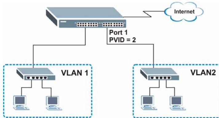
Figure 20 Initial Setup Network Example: Port VID
