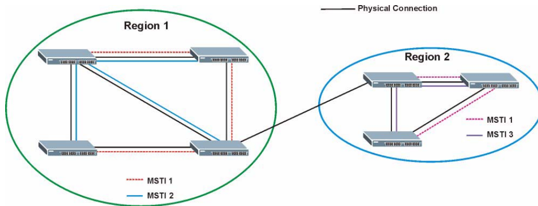
Figure 77 MSTIs in Different Regions
