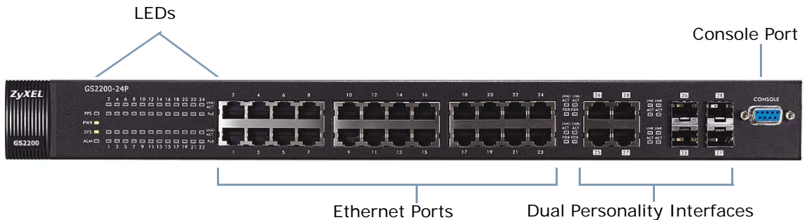
Figure 8 Front Panel (GS200-24P)
