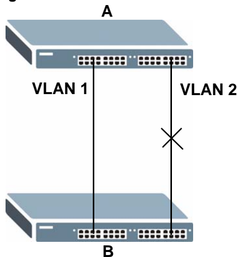
Figure 75 STP/RSTP Network Example
