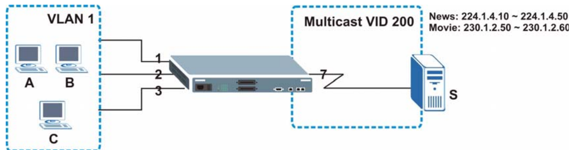
Figure 106 MVR Configuration Example
