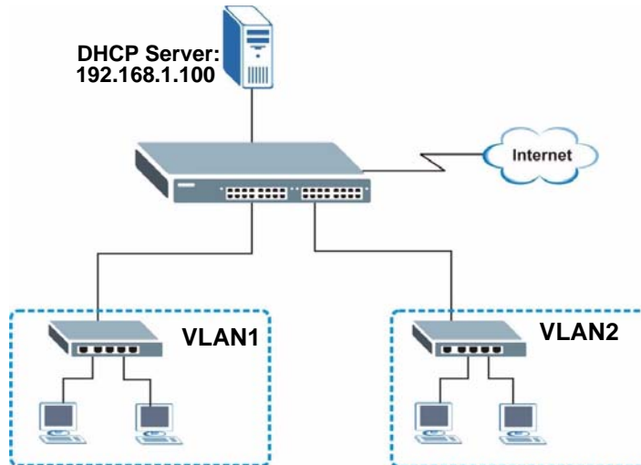
Figure 145 Global DHCP Relay Network Example
