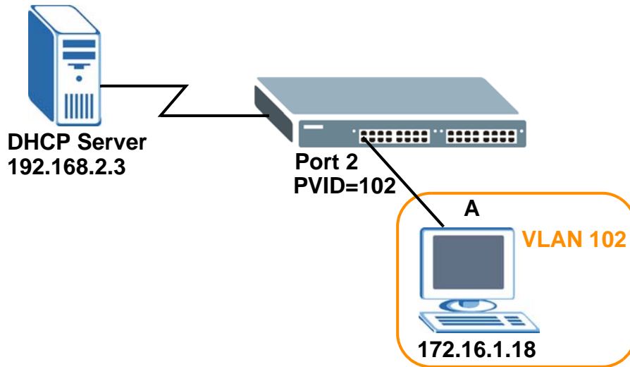
Figure 29 Tutorial: DHCP Relay Scenario
