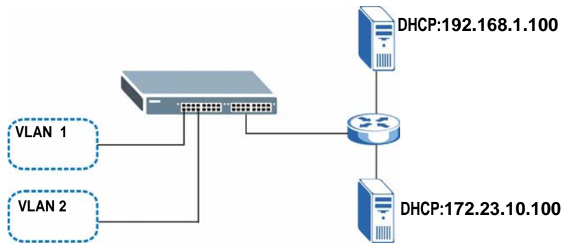
Figure 148 DHCP Relay for Two VLANs
