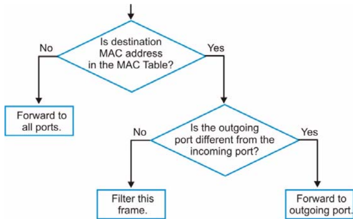
Figure 178 MAC Table Flowchart
