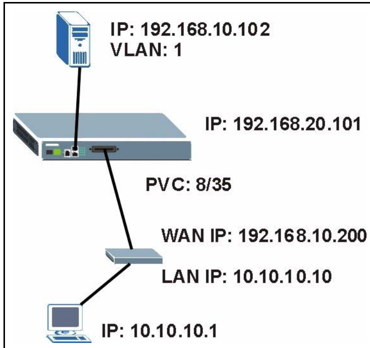
Figure 93 2684 Routed Mode Example
