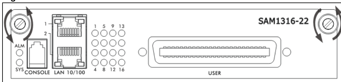
Figure 5 Removal: Loosen Module Screws
