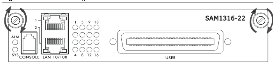
Figure 4 Installation: Tighten Module Screws
