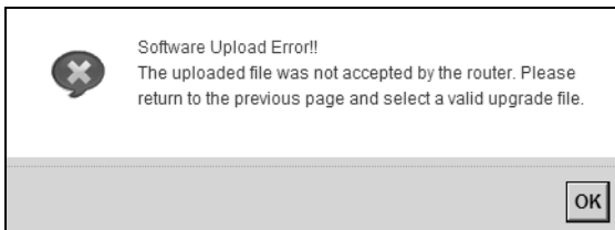
Figure 67 Error Message
