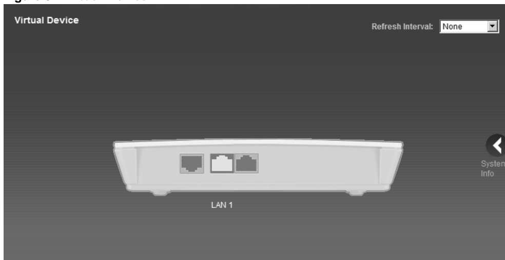
Figure 8 Virtual Device
