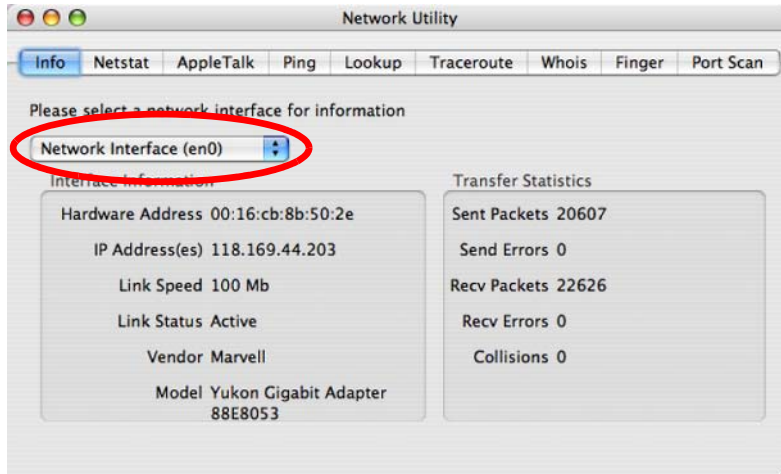
Figure 75 Mac OS X 10.4: Network Utility
