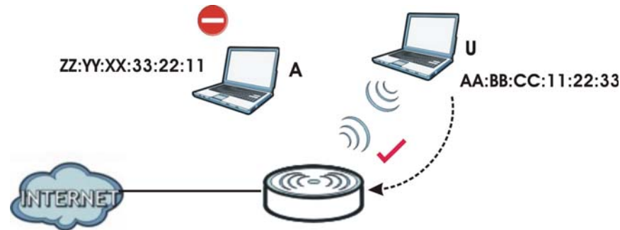
Figure 38 MAC Filtering
