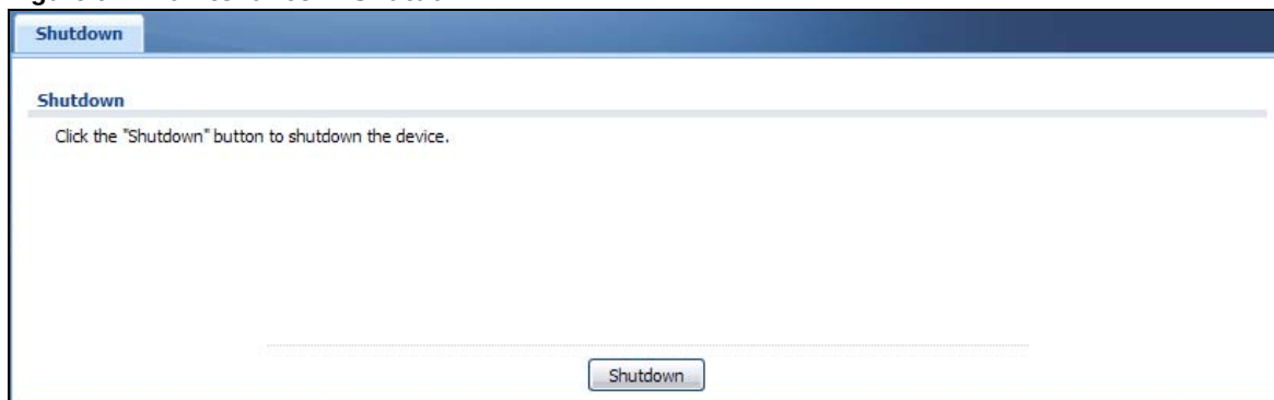
Figure 94 Maintenance > Shutdown
