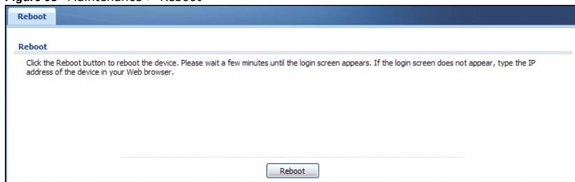
Figure 93 Maintenance > Reboot
