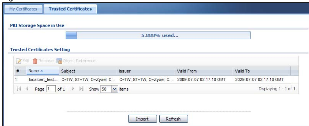
Figure 71 Trusted Certificates
