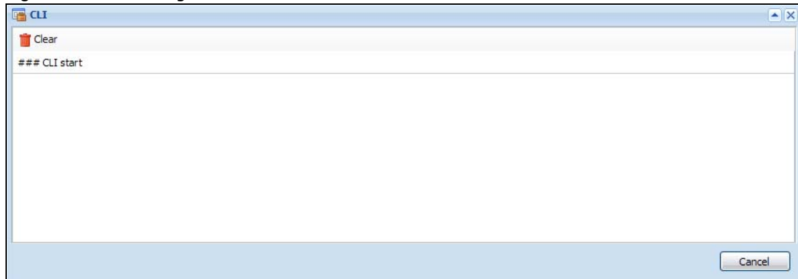
Figure 10 CLI Messages
