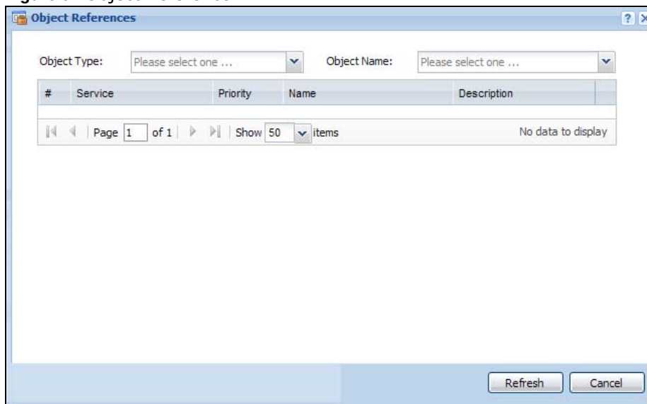
Figure 9 Object Reference
