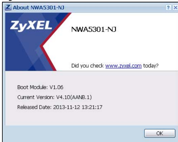
Figure 7 About
