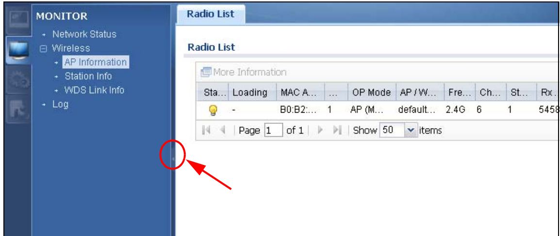
Figure 11 Navigation Panel
