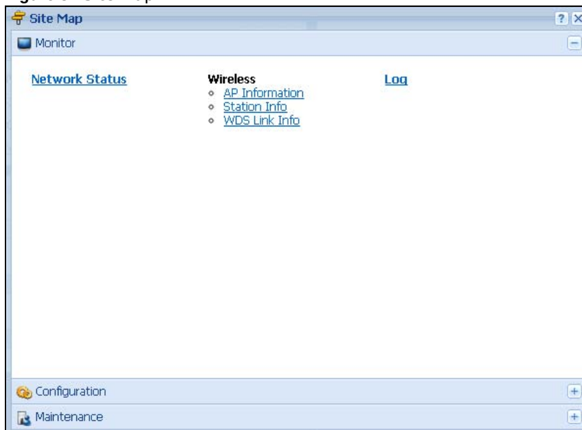
Figure 8 Site Map
