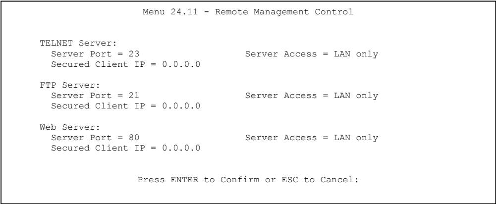
Figure 24-2 Remote Management
