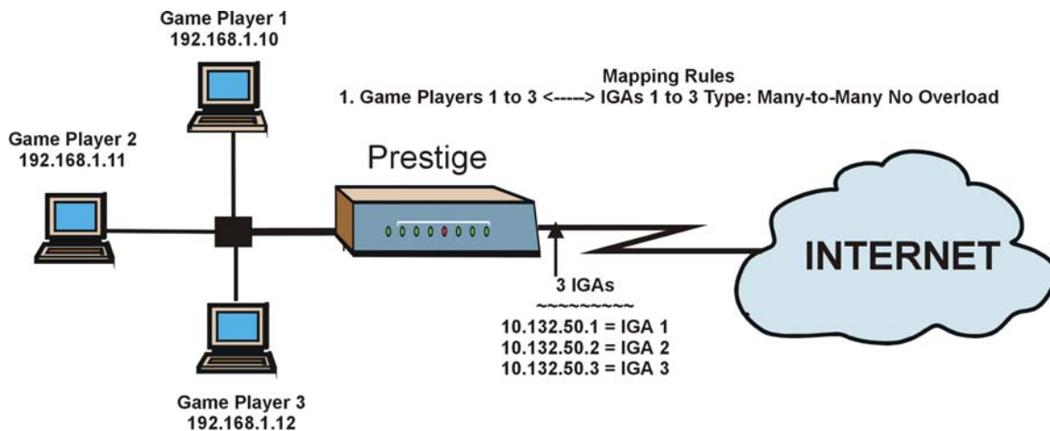
Figure 11-21 NAT Example 4
