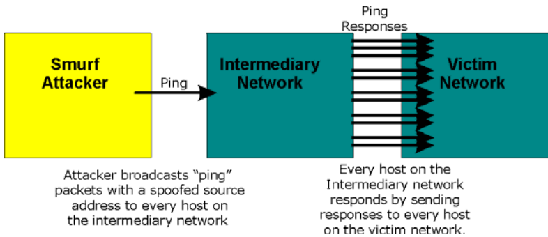
Figure 12-4 Smurf Attack
