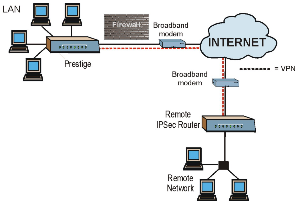
Figure 25-2 VPN Application
