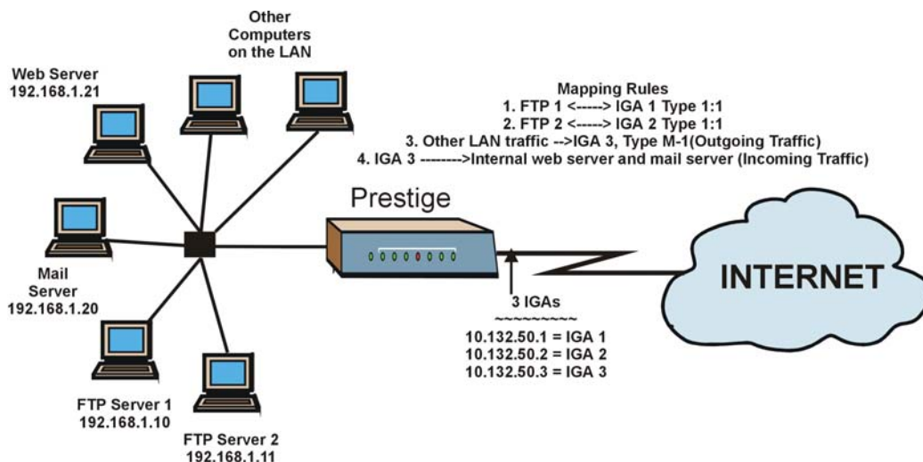
Figure 11-17 NAT Example 3
