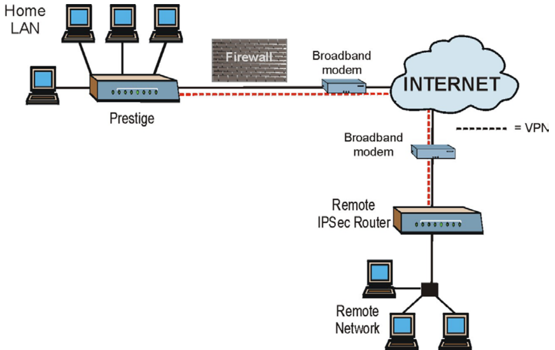
Figure 1-4 Secure Internet Access and VPN Application
