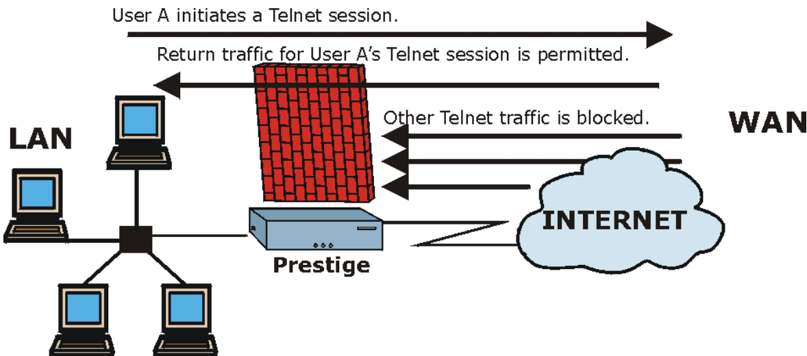
Figure 12-5 Stateful Inspection
