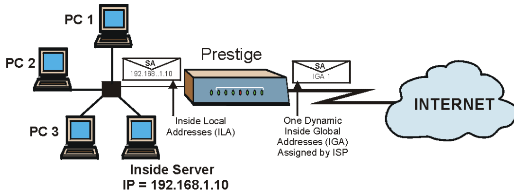
Figure 11-15 NAT Example 2
