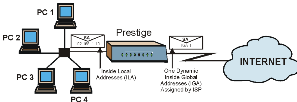
Figure 11-13 NAT Example 1
