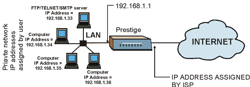
Figure 11-12 Multiple Servers Behind NAT Example
