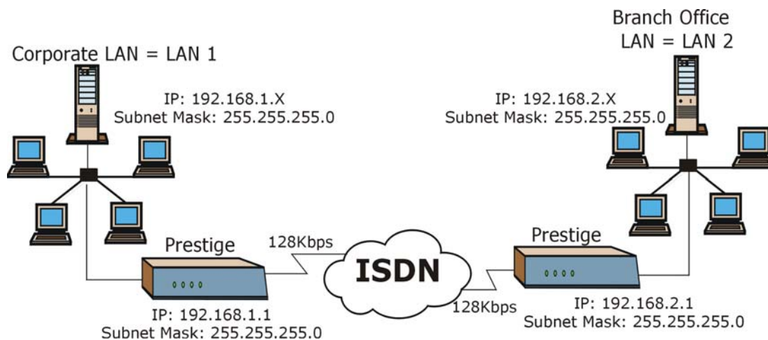
Figure 8-4 TCP/IP LAN-to-LAN Application
