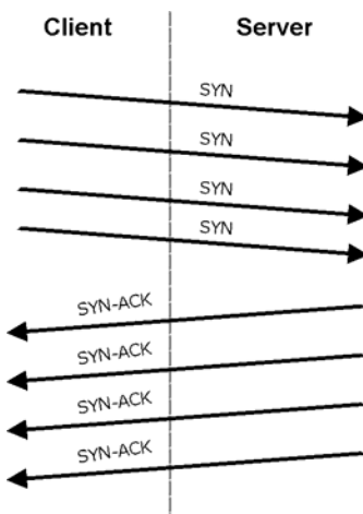
Figure 12-3 SYN Flood
