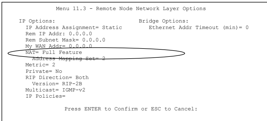
Figure 11-18 Example 3: Menu 11.3
