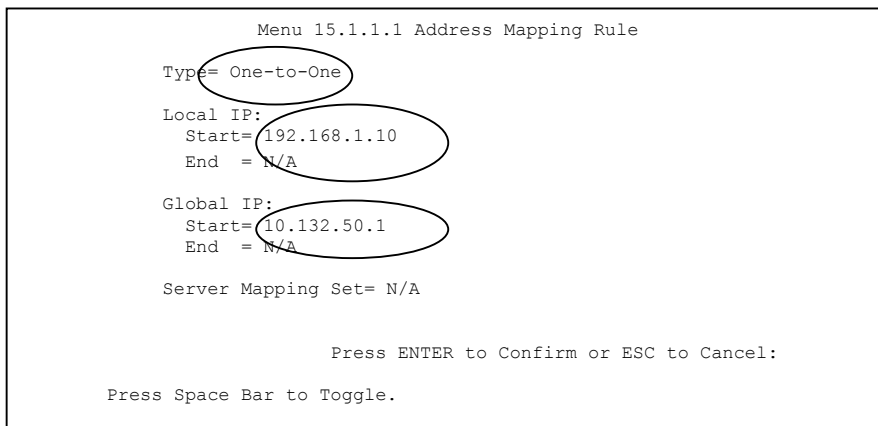
Figure 11-19 Example 3: Menu 15.1.1.1
