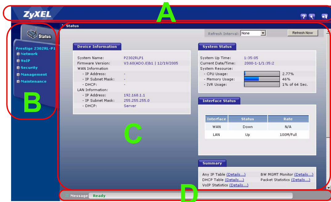
Figure 8 Main Screen
