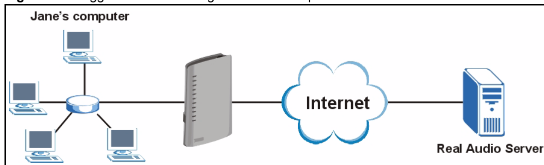
Figure 48 Trigger Port Forwarding Process: Example
