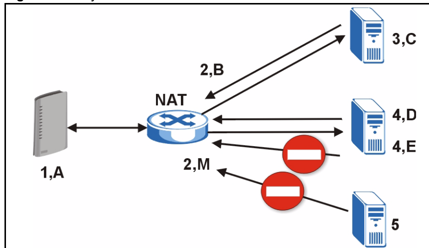
Figure 146 Symmetric NAT
