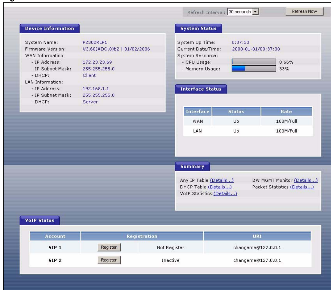
Figure 29 Status Screen
