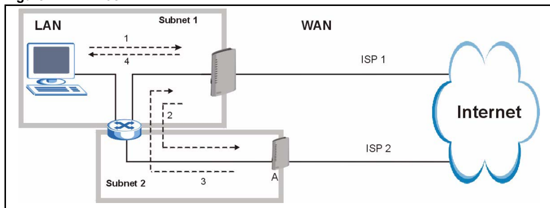
Figure 72 IP Alias
