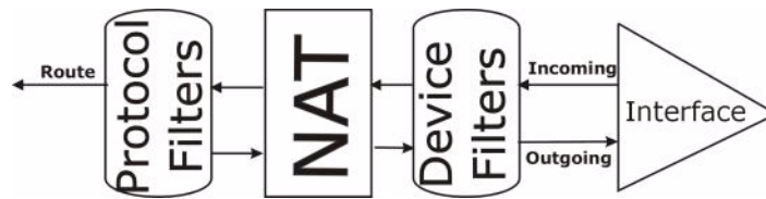
Figure 203 Protocol and Device Filter Sets
