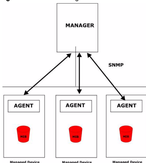
Figure 125 SNMP Management Model
