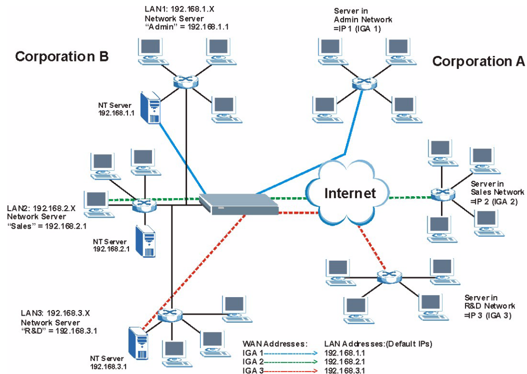
Figure 65 NAT Application With IP Alias
