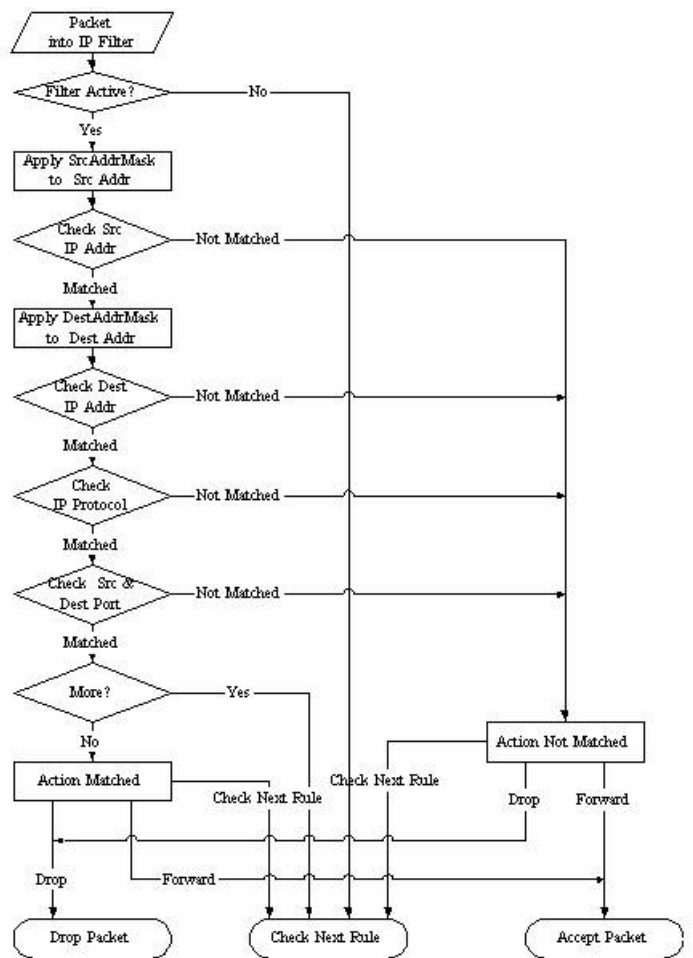
Figure 198 Executing an IP Filter
