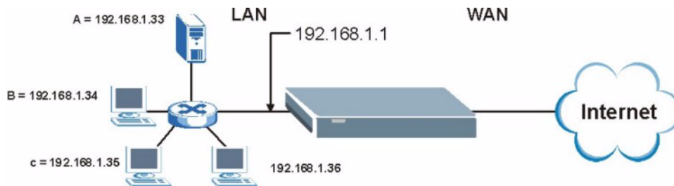
Figure 66 Multiple Servers Behind NAT Example
