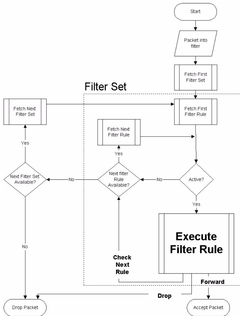
Figure 194 Filter Rule Process
