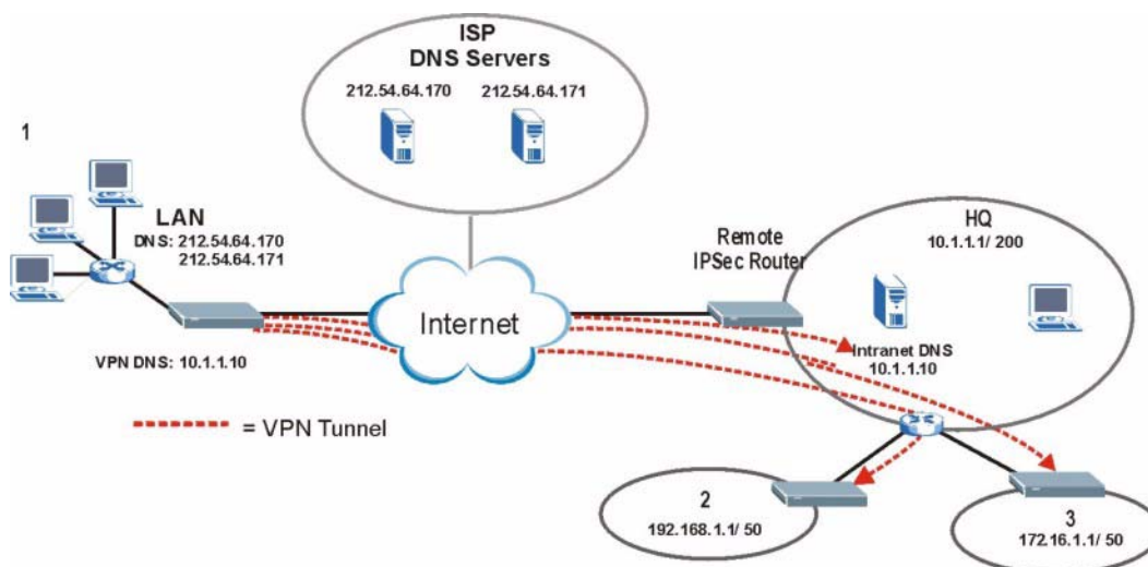
Figure 83 VPN Host using Intranet DNS Server Example
