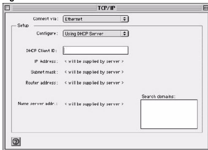
Figure 266 Macintosh OS 8/9: TCP/IP
