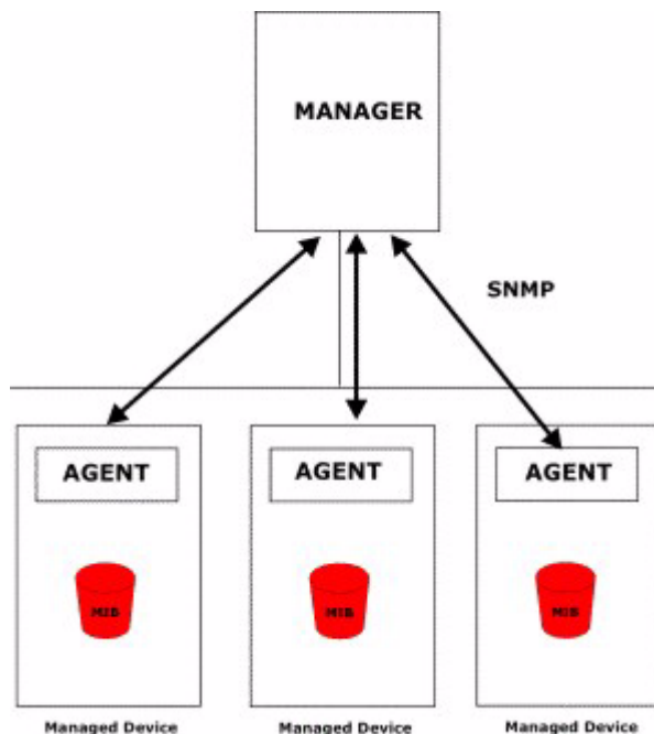
Figure 206 SNMP Management Model
