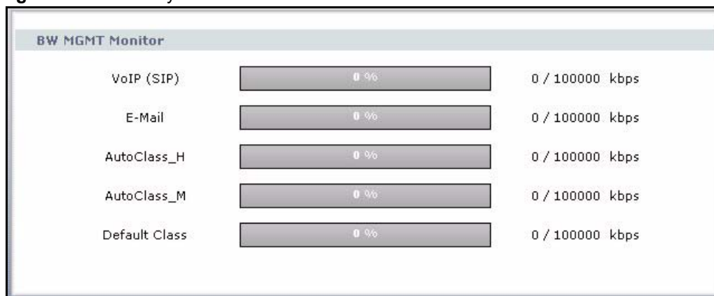
Figure 11 Summary: BW MGMT Monitor
