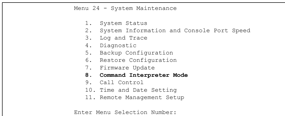
Figure 227 Command Mode in Menu 24
