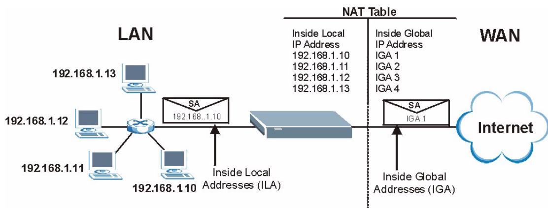
Figure 64 How NAT Works
