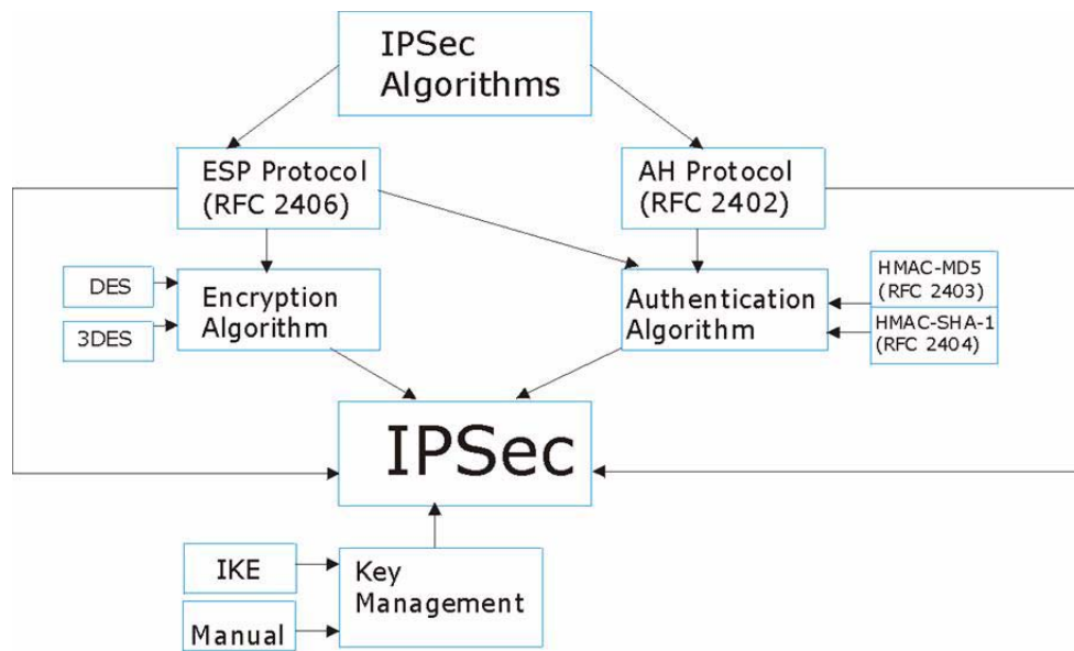
Figure 78 IPSec Architecture
