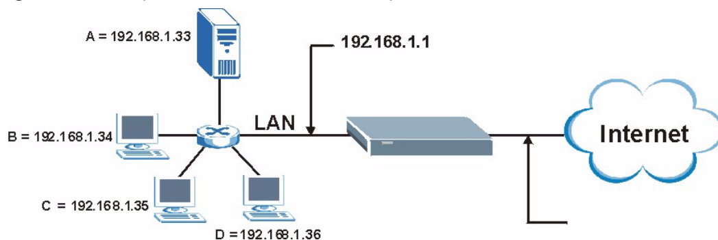
Figure 178 Multiple Servers Behind NAT Example
