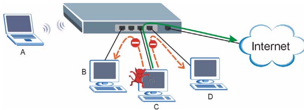
Figure 110 Port Isolation Example
