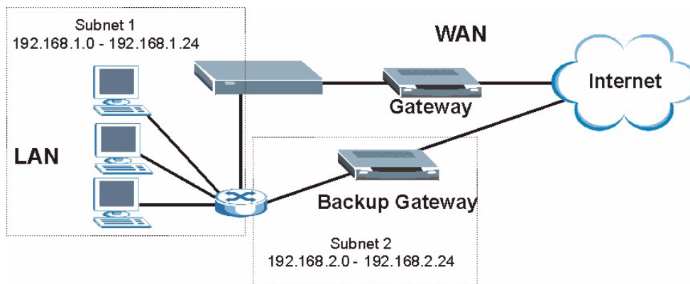
Figure 55 Traffic Redirect LAN Setup
