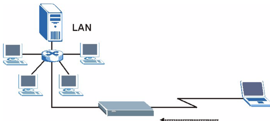
Figure 200 Telnet Filter Example
