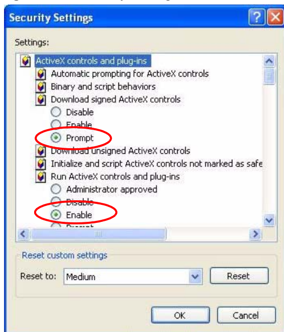
Figure 254 Security Setting ActiveX Controls
