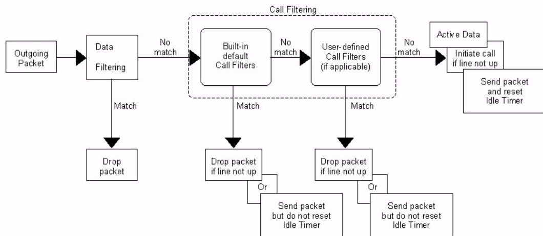
Figure 193 Outgoing Packet Filtering Process
