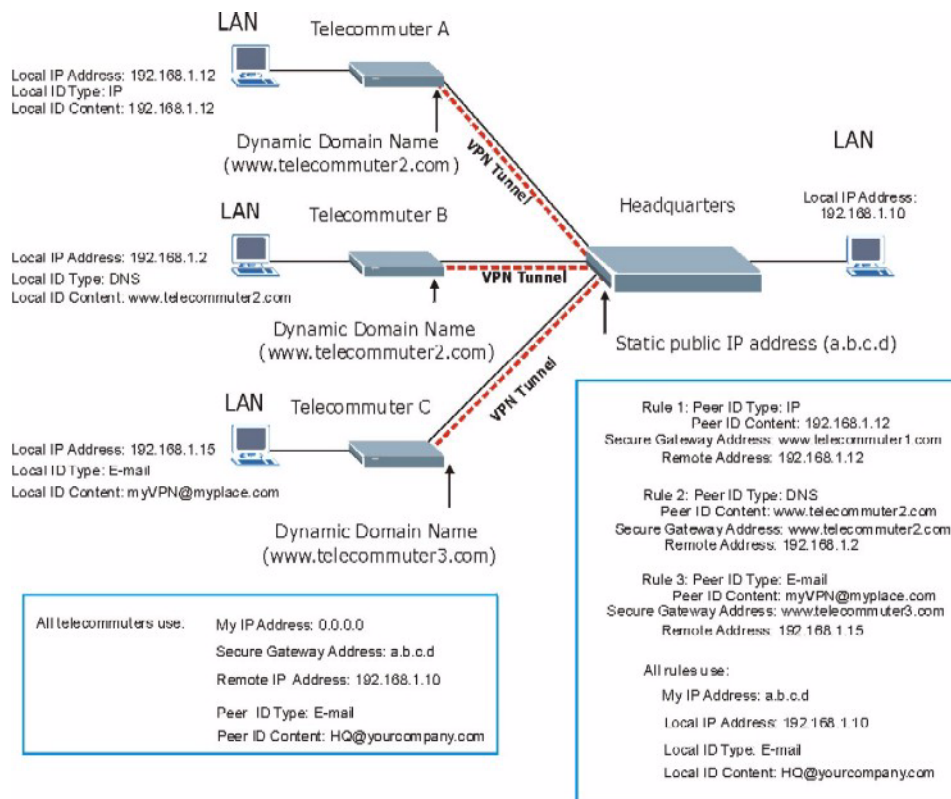
Figure 92 Telecommuters Using Unique VPN Rules Example
