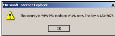
Figure 44 OTIST Start
