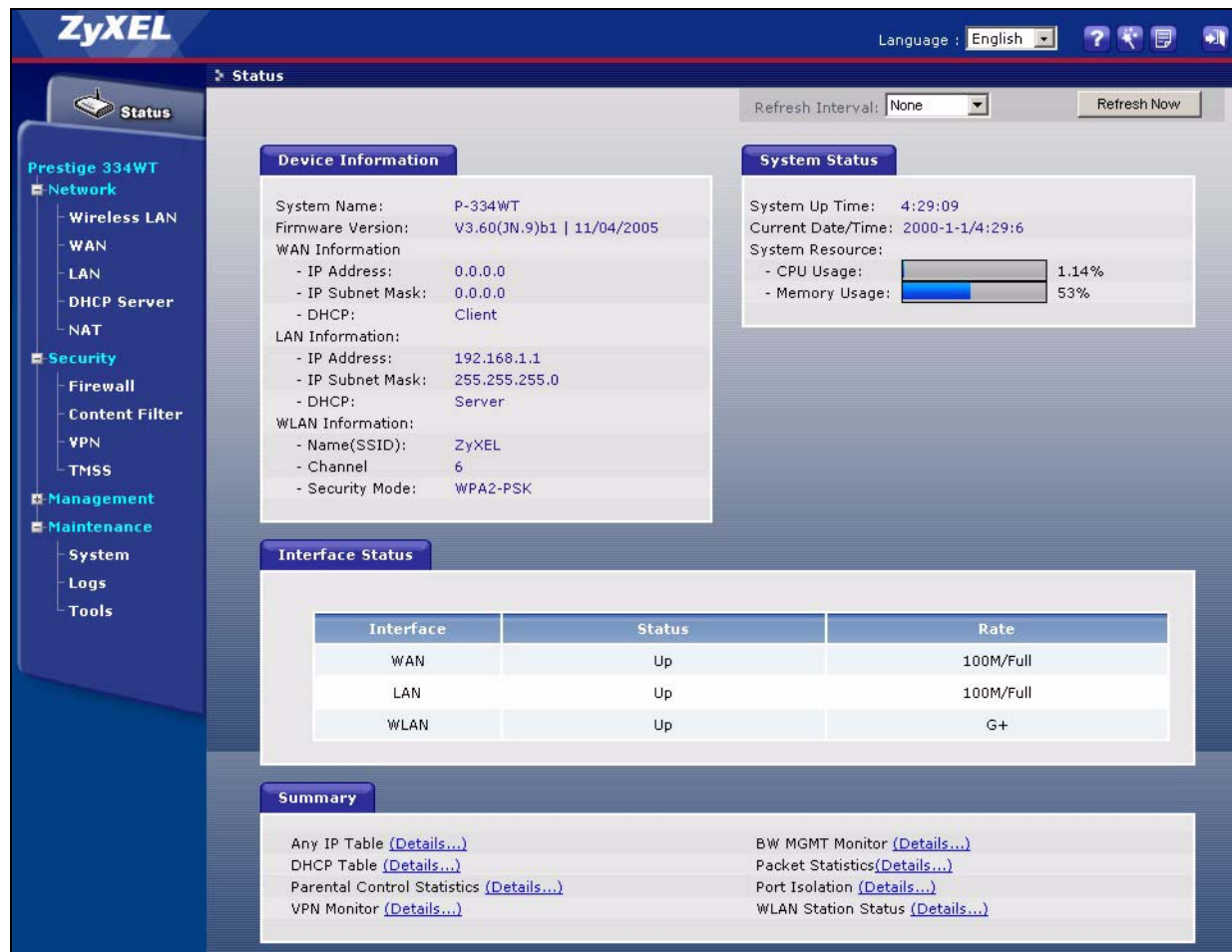
Figure 6 Web Configurator Status Screen
