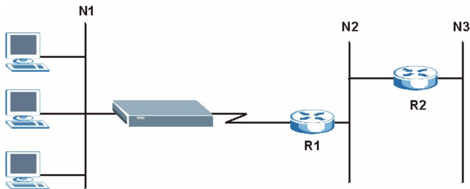
Figure 112 Example of Static Routing Topology
