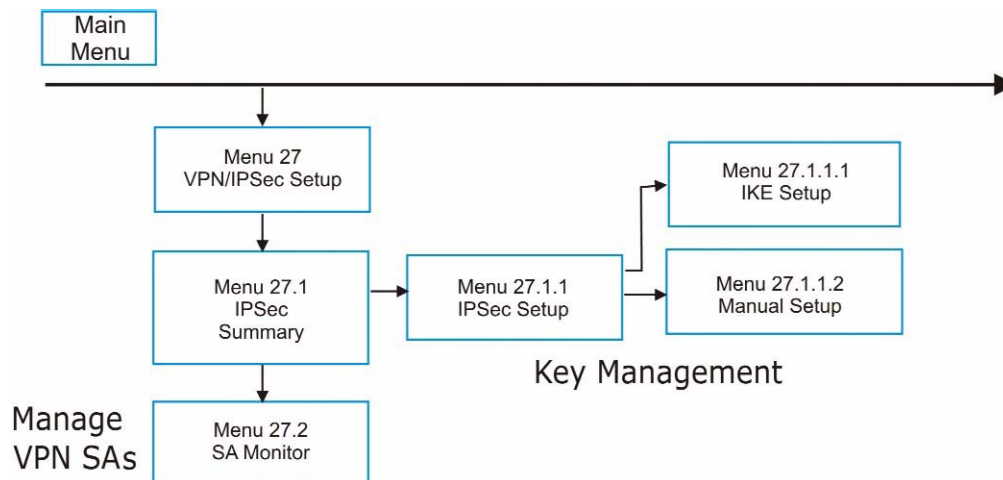
Figure 238 VPN SMT Menu Tree
