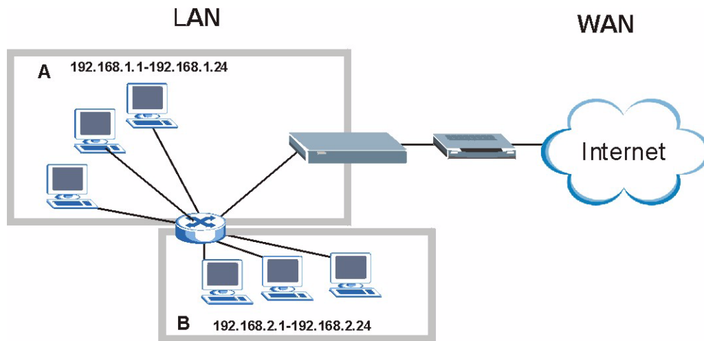
Figure 115 Subnet-based Bandwidth Management Example
