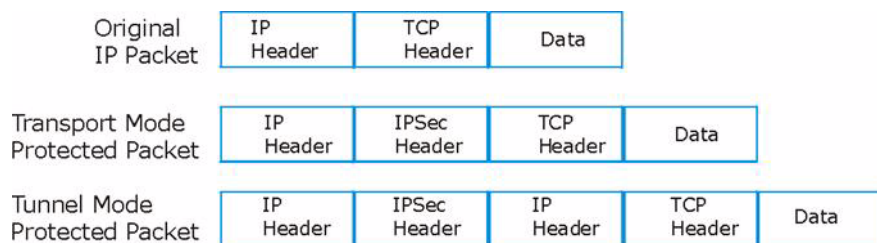
Figure 79 Transport and Tunnel Mode IPSec Encapsulation
