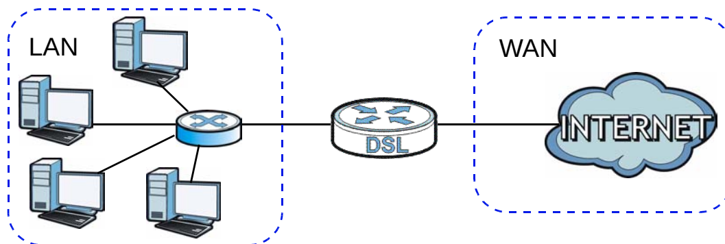
Figure 39 LAN and WAN IP Addresses
