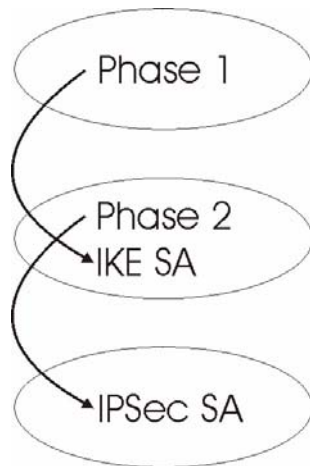
Figure 81 Two Phases to Set Up the IPSec SA
