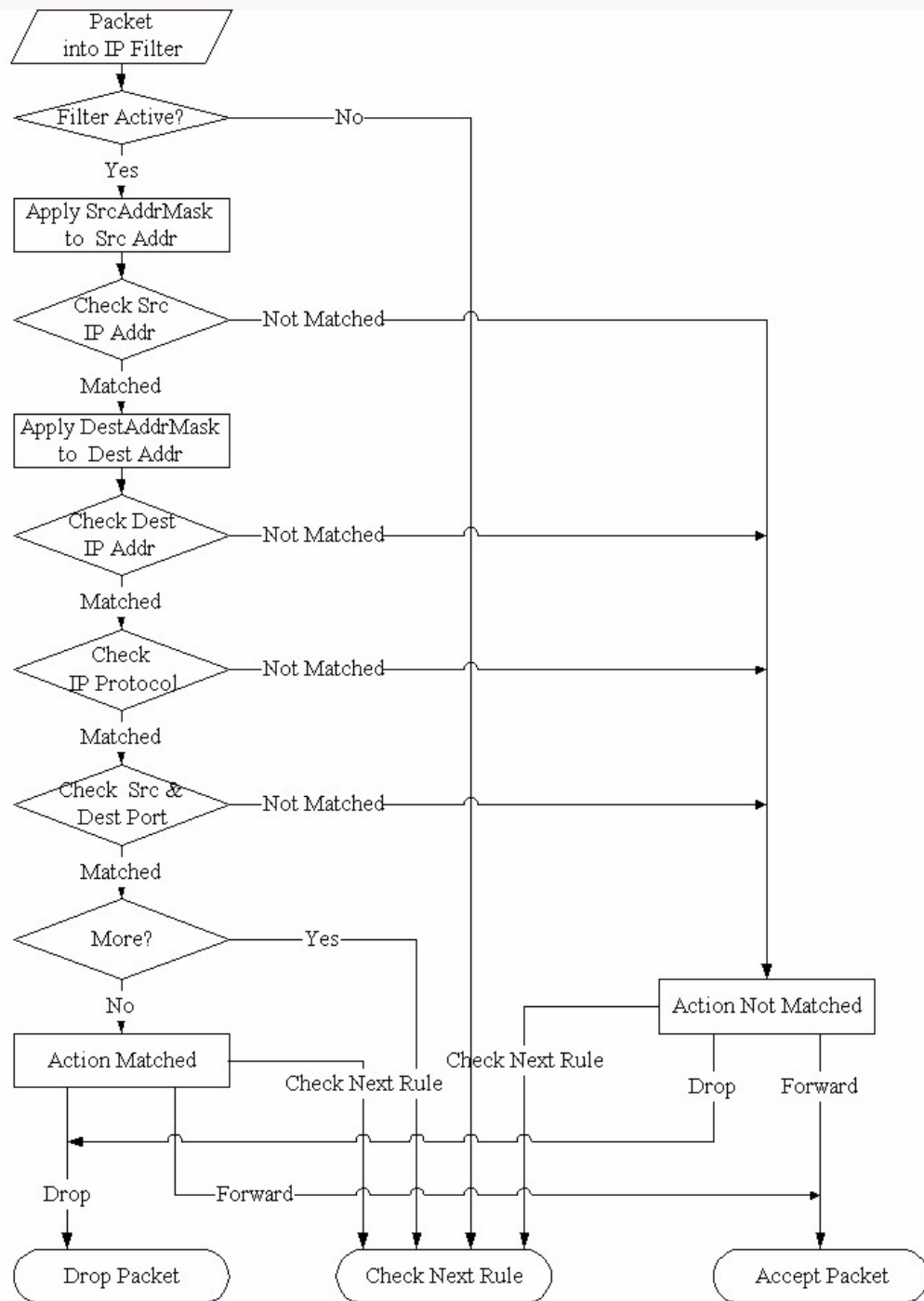
Figure 180 Executing an IP Filter
