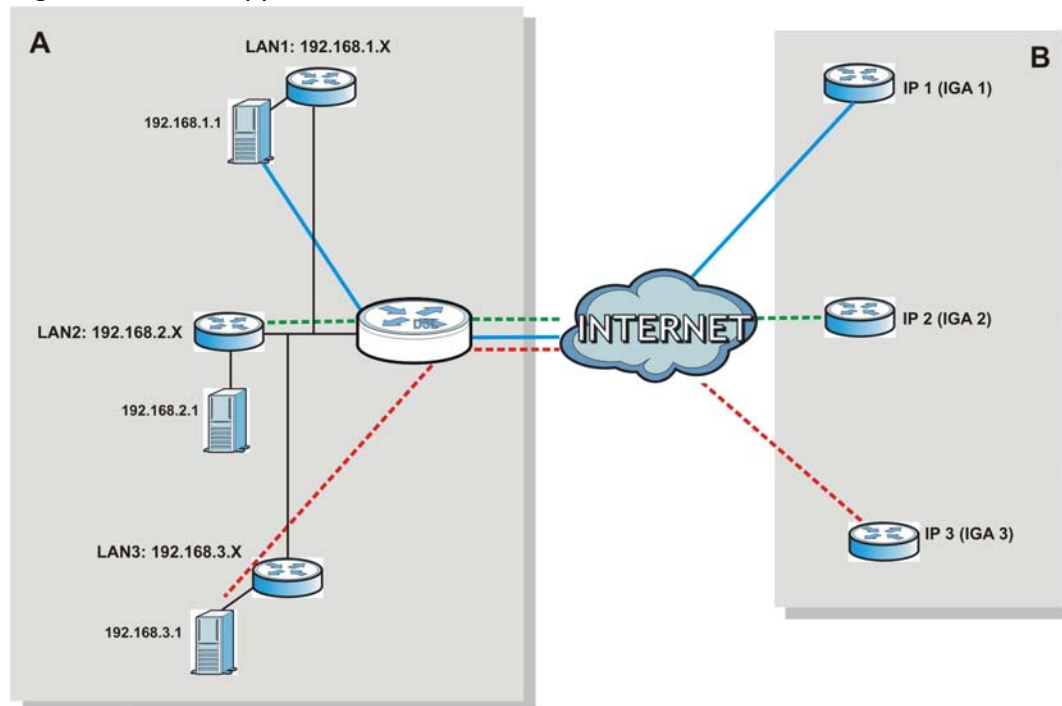
Figure 48 NAT Application With IP Alias
