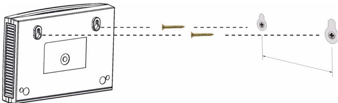
Figure 227 Wall-mounting Example
