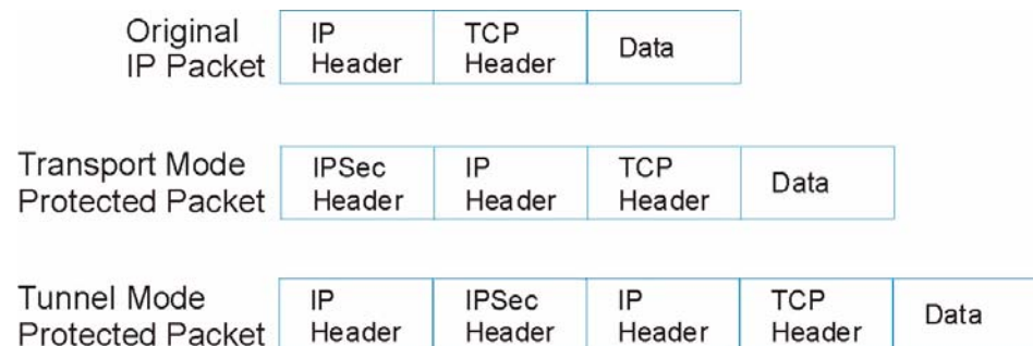
Figure 80 Transport and Tunnel Mode IPSec Encapsulation
