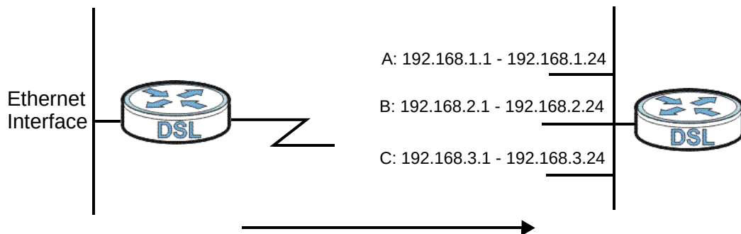
Figure 37 Physical Network & Partitioned Logical Networks
