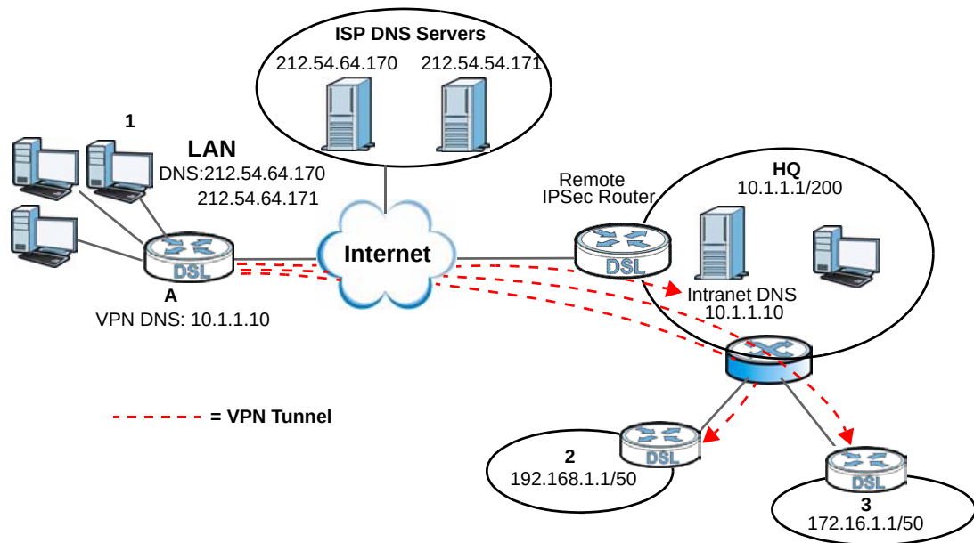
Figure 82 VPN Host using Intranet DNS Server Example
