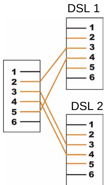
Figure 226 Y-Cable Configuration
