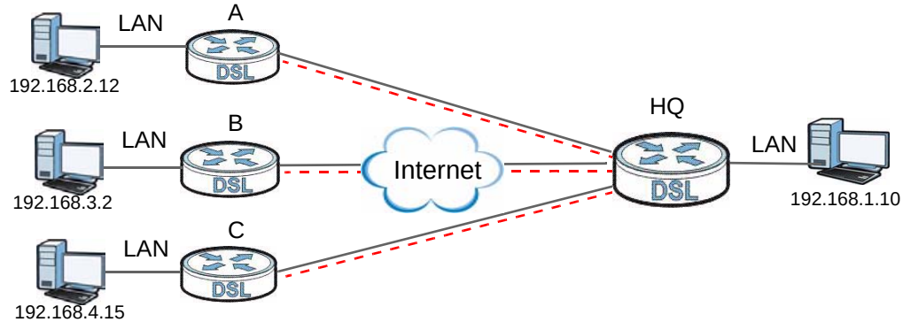
Figure 84 Telecommuters Using Unique VPN Rules Example
