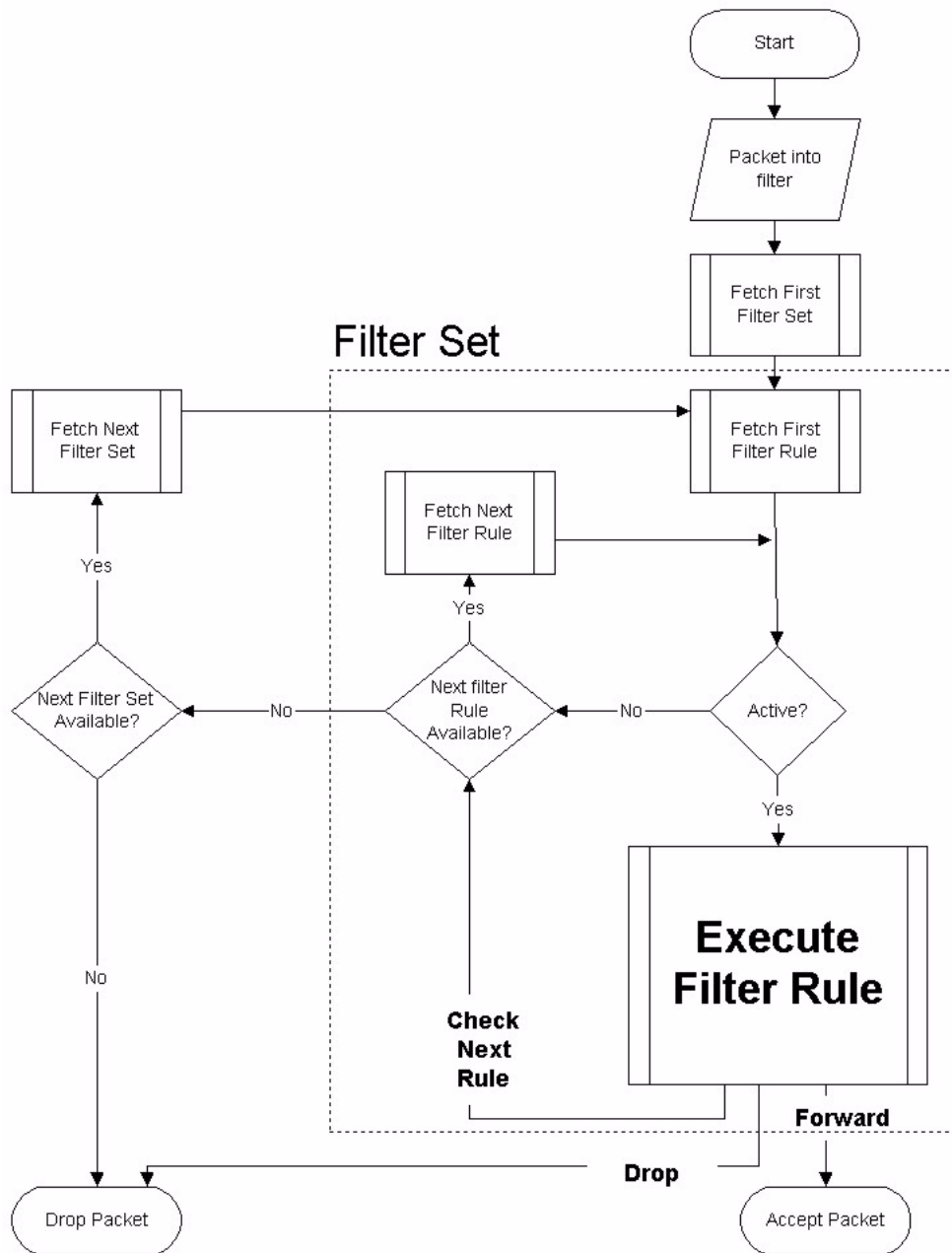
Figure 175 Filter Rule Process
