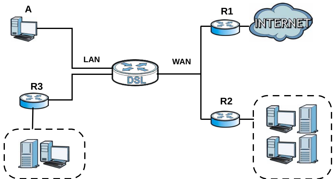
Figure 85 Example of Static Routing Topology
