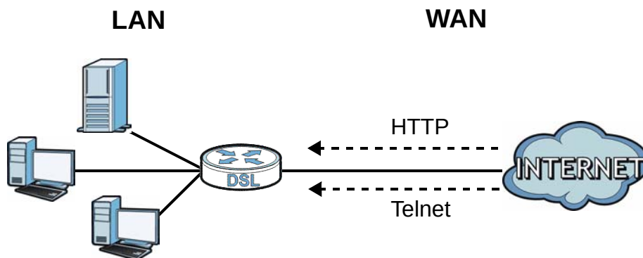
Figure 102 Remote Management From the WAN
