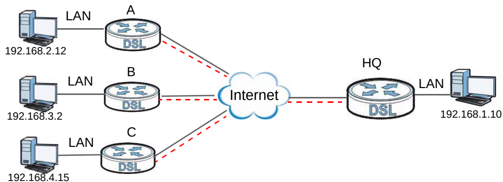
Figure 83 Telecommuters Sharing One VPN Rule Example
