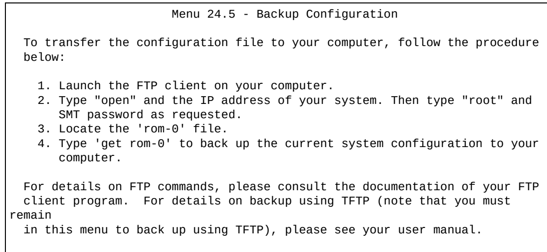
Figure 198 Menu 24.5: Backup Configuration
