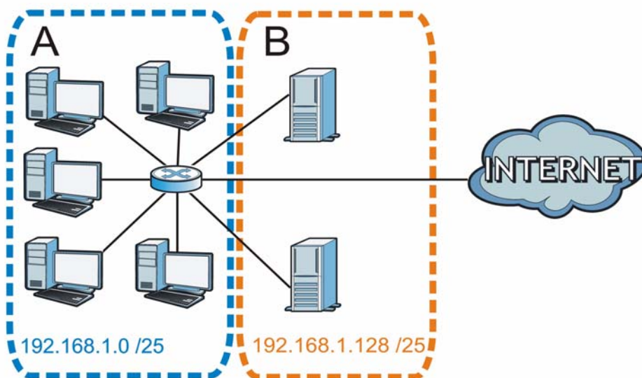
Figure 272 Subnetting Example: After Subnetting
