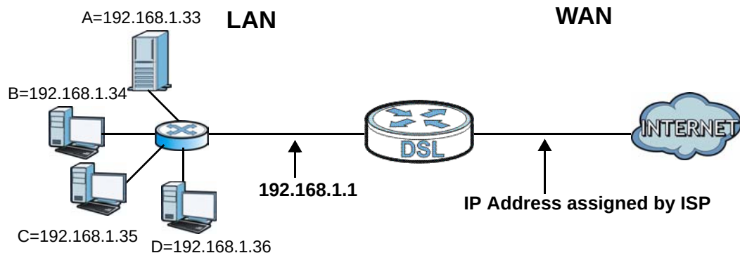
Figure 41 Multiple Servers Behind NAT Example
