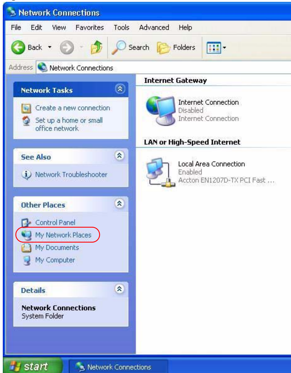
Figure 116 Network Connections
