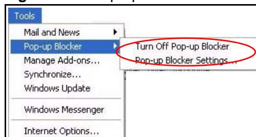
Figure 181 Pop-up Blocker
