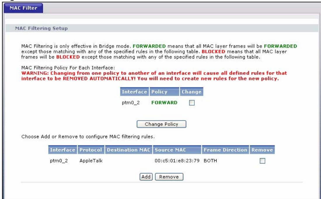
Figure 73 MAC Filter
