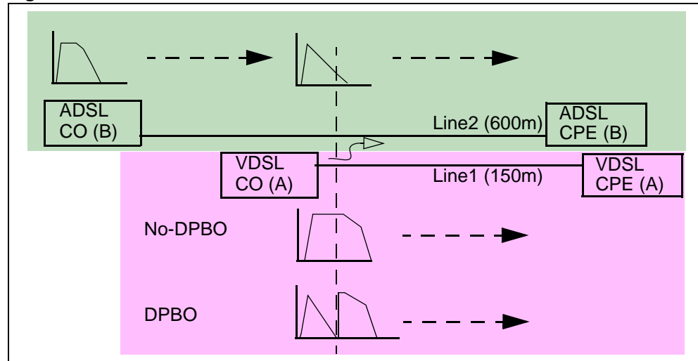
Figure 46 DPBO Resolves Downstream Far-End Crosstalk
