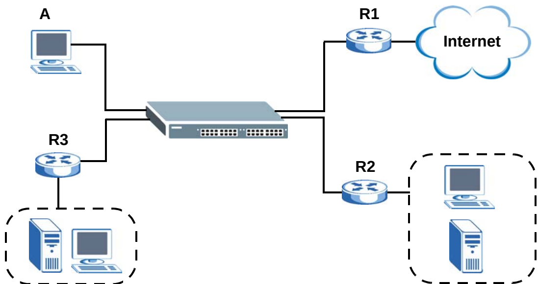
Figure 157 Example of Static Routing Topology
