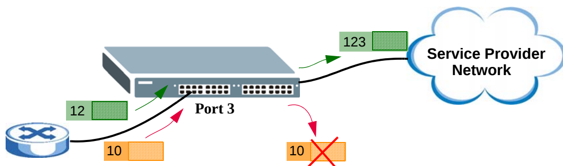
Figure 139 VLAN mapping example
