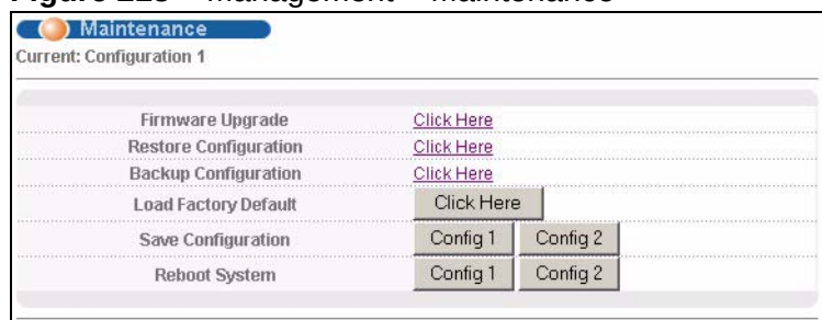
Figure 213 Management > Maintenance
