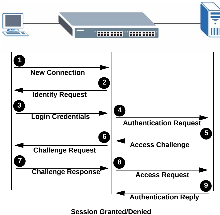
Figure 83 IEEE 802.1x Authentication Process
