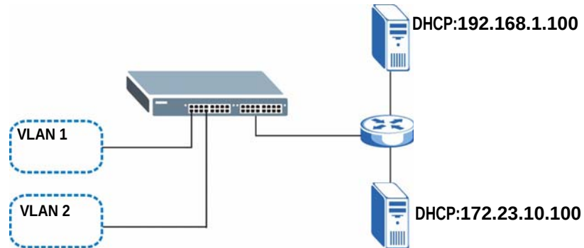
Figure 194 DHCP Relay for Two VLANs
