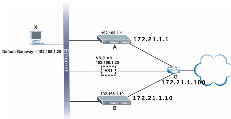
Figure 196 VRRP: Example 1
