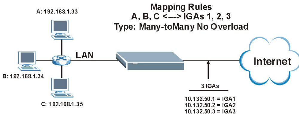
Figure 28-19 NAT Example 4
