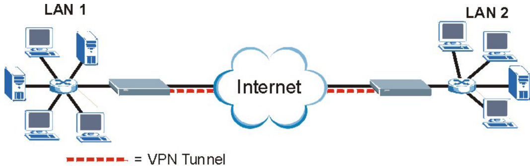
Figure 14-6 Site-to-Site VPN Example
