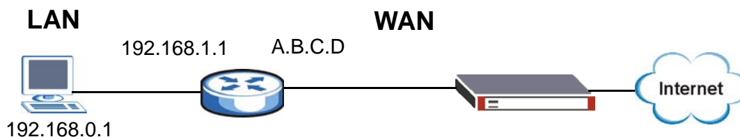
Figure 90 Router Mode
