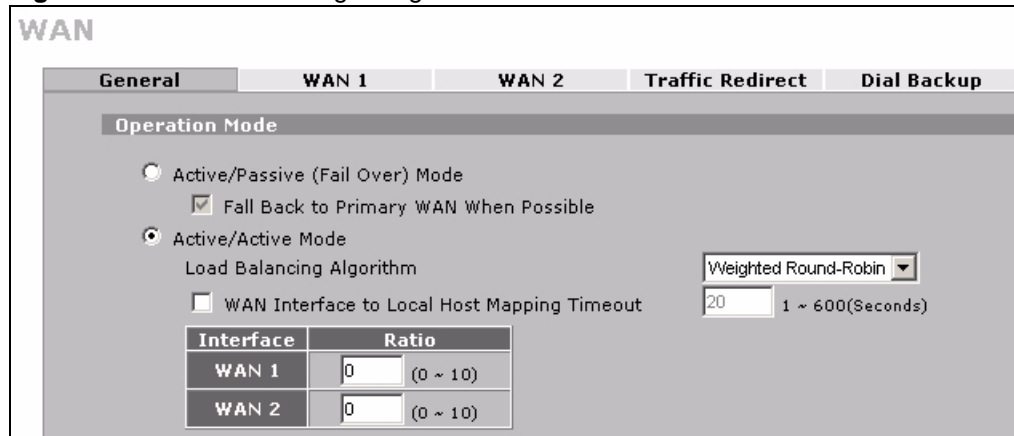
Figure 102 Load Balancing: Weighted Round Robin
