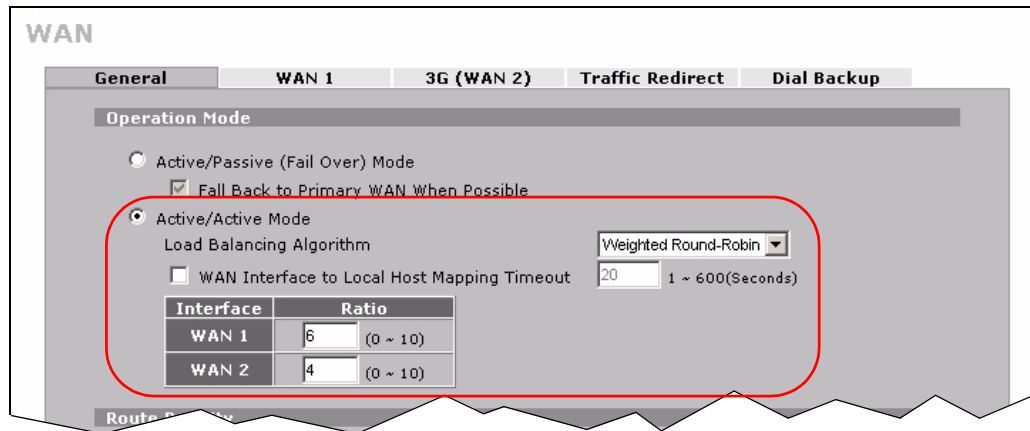
Figure 68 Tutorial: NETWORK &gt; WAN &gt; General
