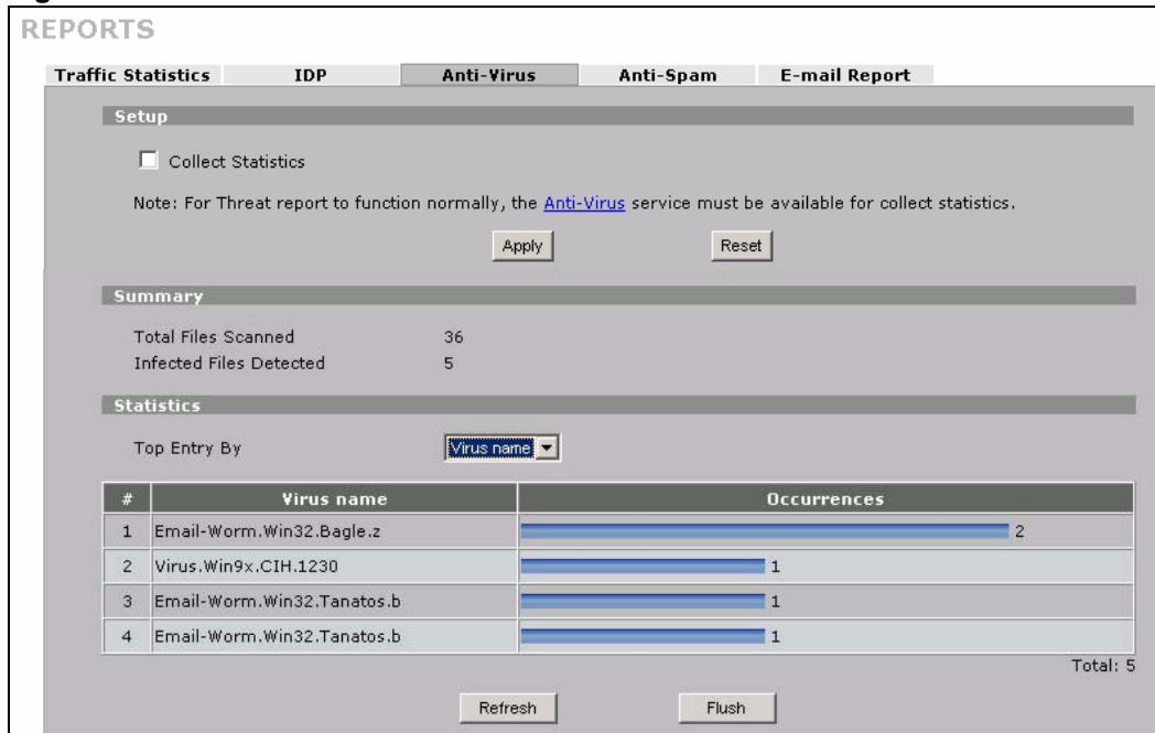
Figure 329 REPORTS > Anti-Virus
