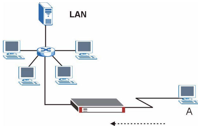
Figure 443 Telnet Filter Example
