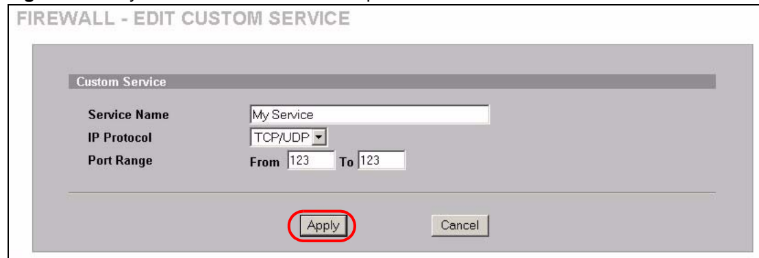
Figure 154 My Service Firewall Rule Example: Edit Custom Service
