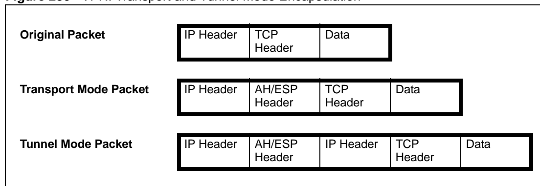
Figure 230 VPN: Transport and Tunnel Mode Encapsulation
