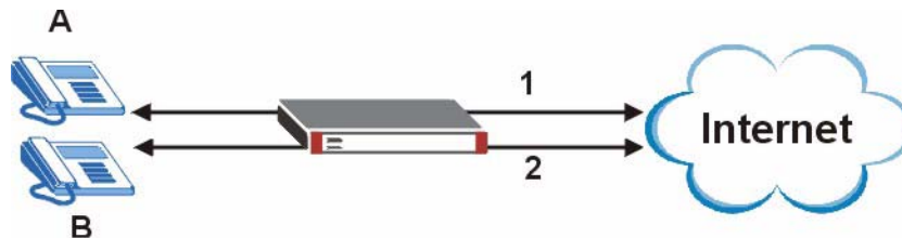
Figure 318 H.323 with Multiple WAN IP Addresses
