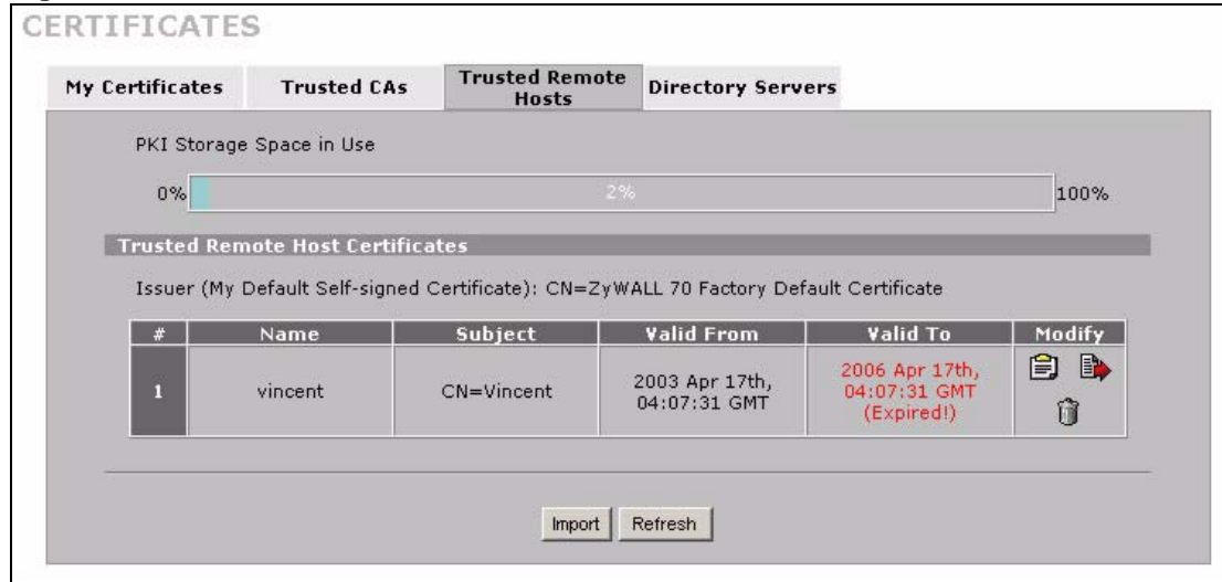
Figure 244 SECURITY > CERTIFICATES > Trusted Remote Hosts
