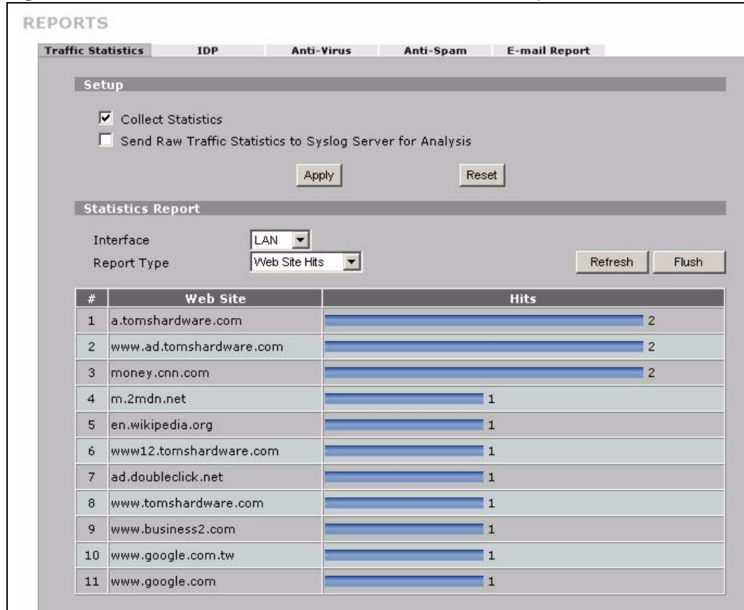
Figure 323 REPORTS > Traffic Statistics: Web Site Hits Example
