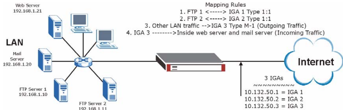
Figure 425 NAT Example 3
