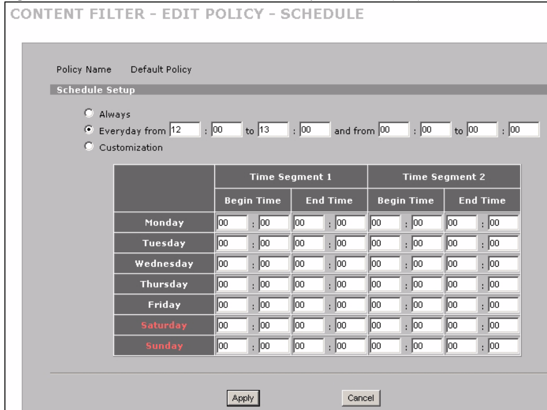
Figure 76 SECURITY > CONTENT FILTER > Policy > Schedule (Bob)
