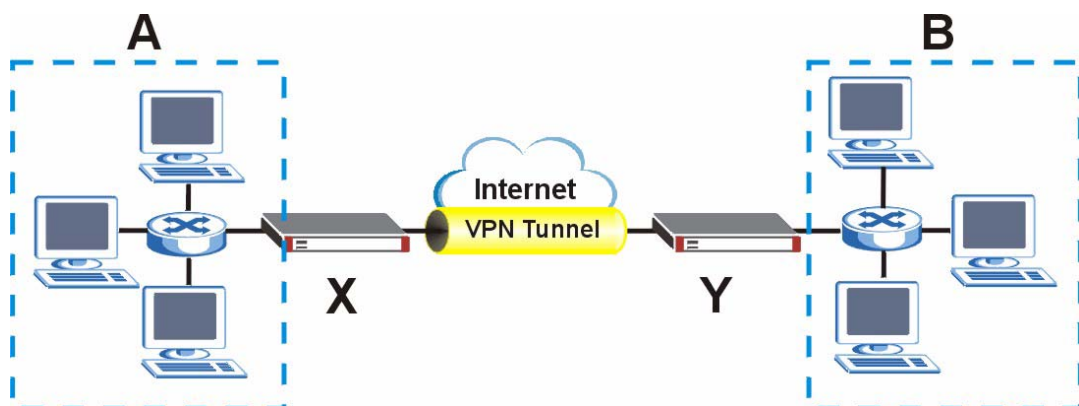
Figure 205 VPN: Example
