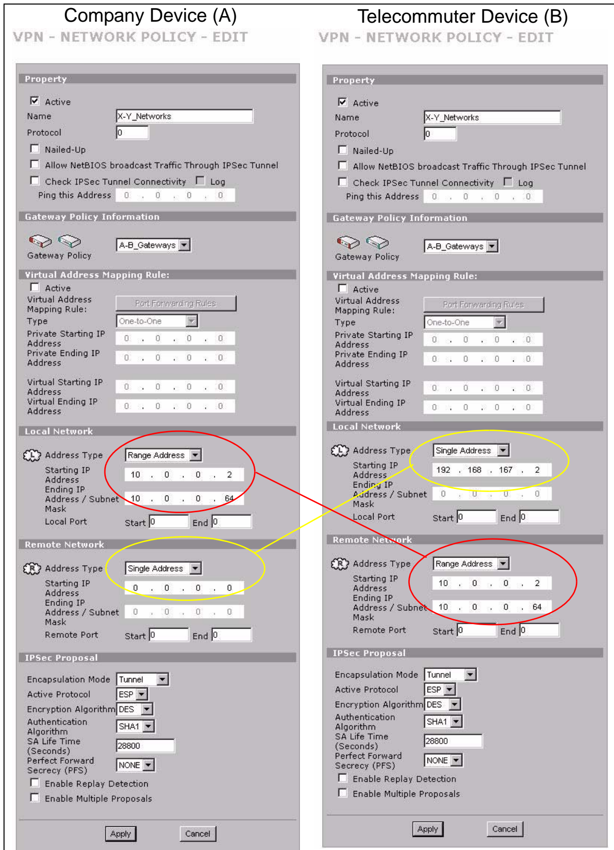
Figure 47 VPN Network Policy Edit Screens
