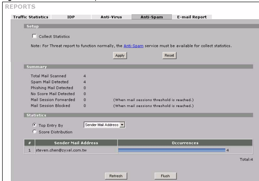
Figure 332 REPORTS > Anti-Spam
