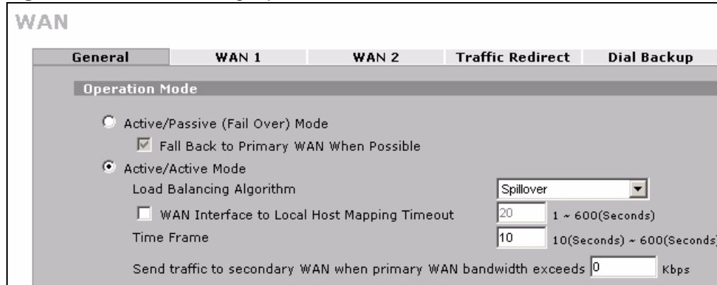
Figure 104 Load Balancing: Spillover
