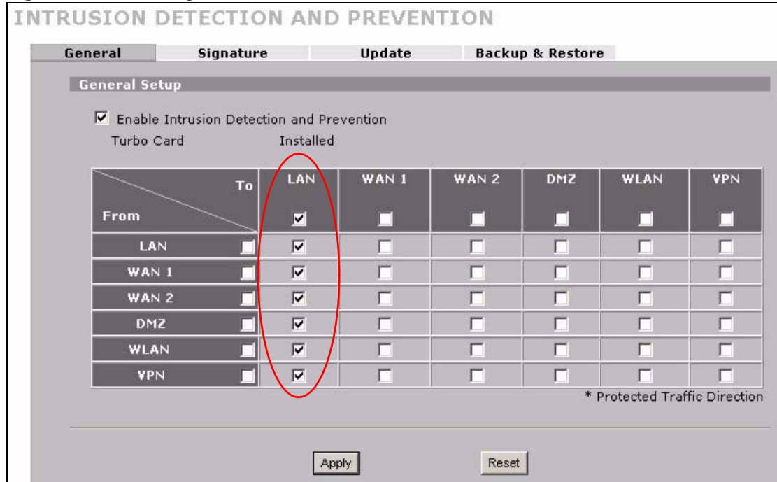
Figure 54 IDP Configuration for Traffic From VPN
