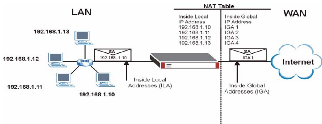
Figure 259 NAT Overview
