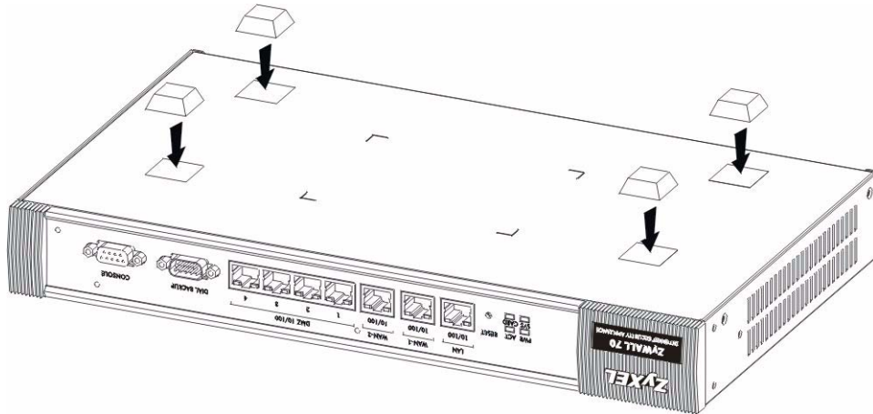
Figure 4 Attaching Rubber Feet
