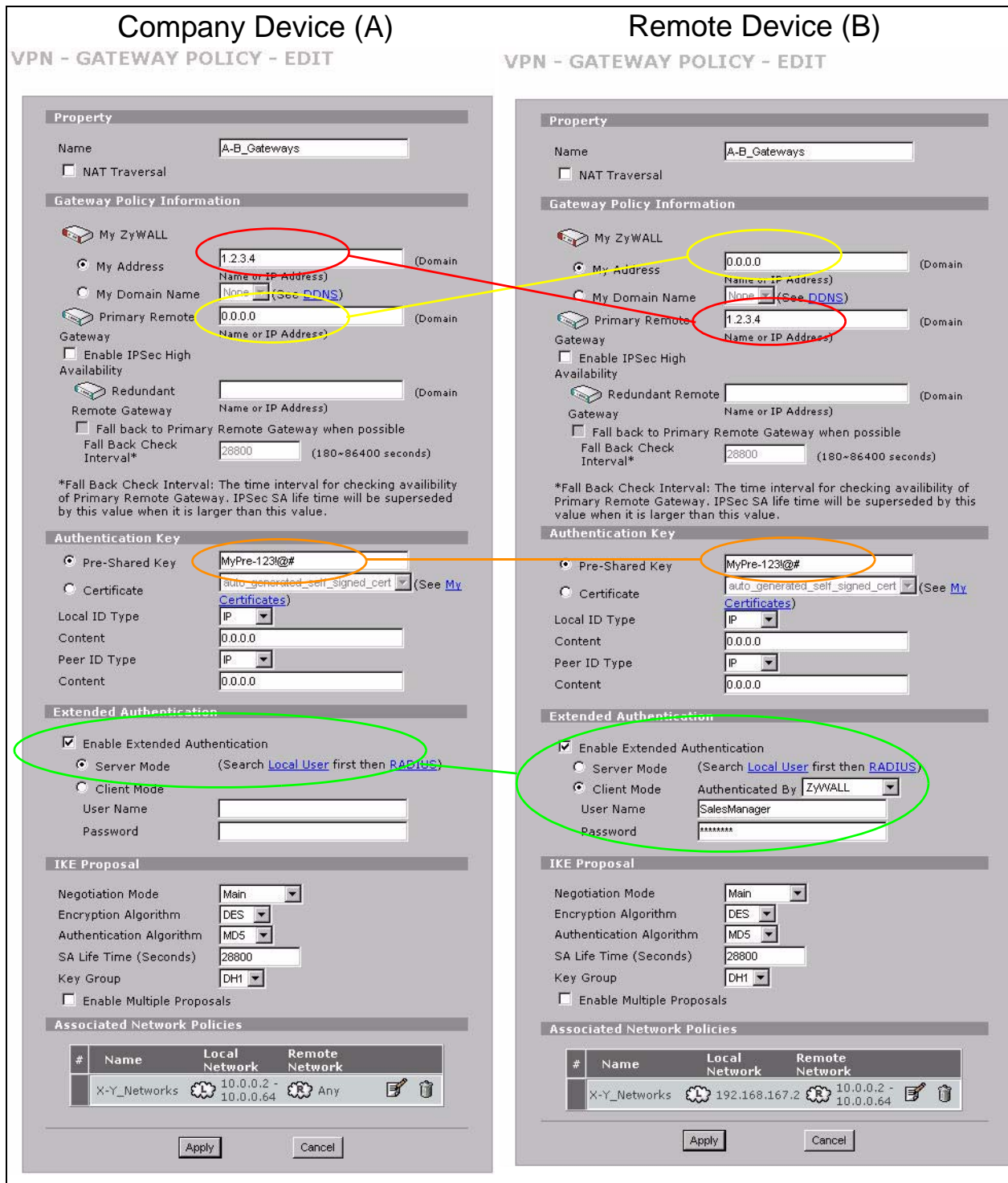
Figure 45 VPN Gateway Policy Edit Screens
