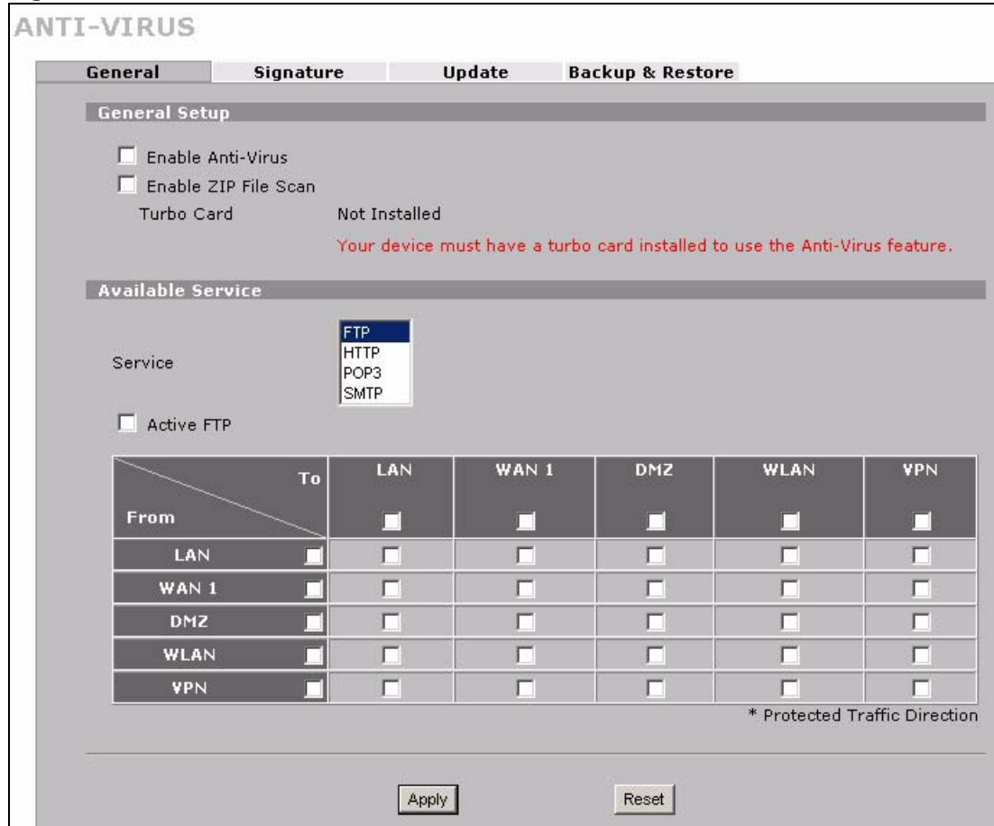
Figure 176 SECURITY > ANTI-VIRUS > General
