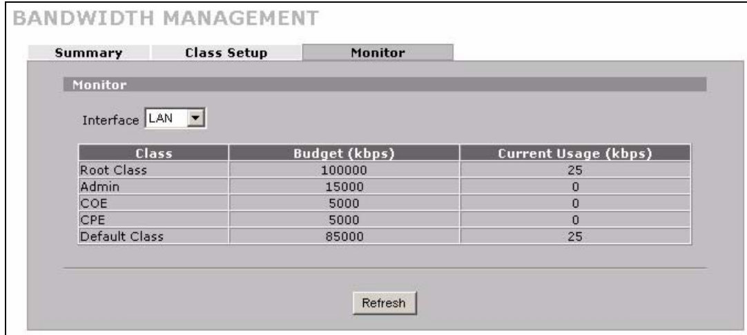
Figure 272 ADVANCED > BW MGMT > Monitor
