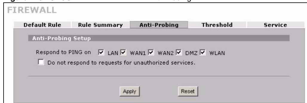
Figure 149 SECURITY > FIREWALL > Anti-Probing
