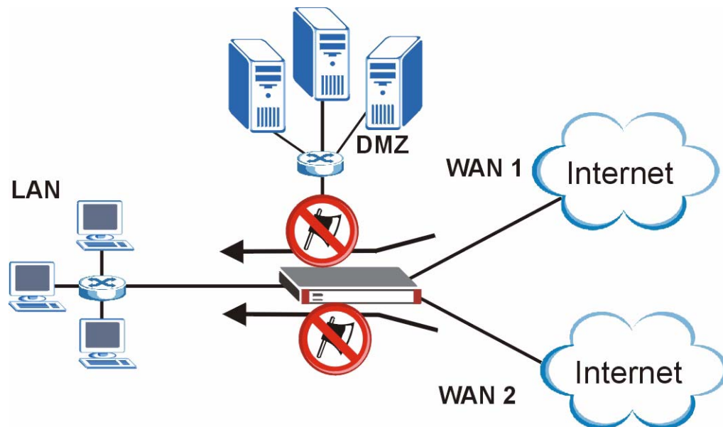
Figure 165 Applying IDP to Interfaces
