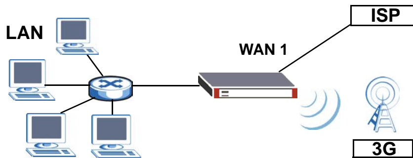
Figure 96 LAN and WAN (Multiple)
