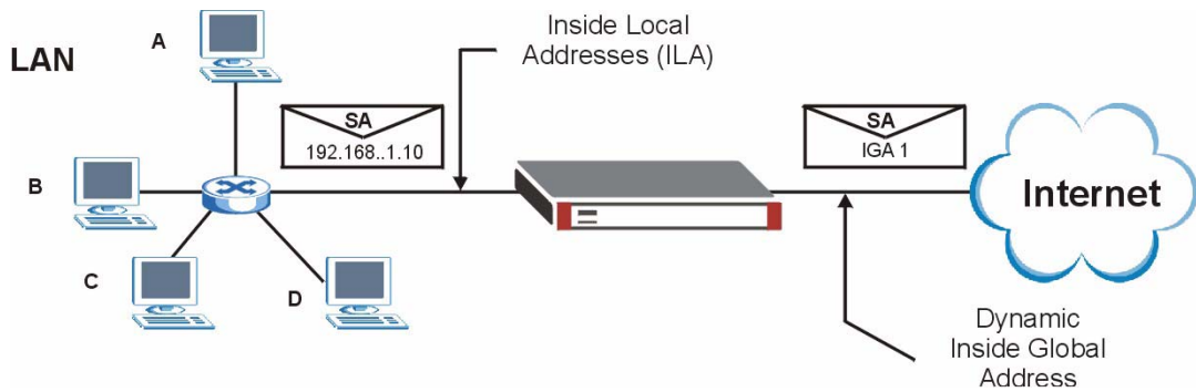
Figure 421 NAT Example 1
