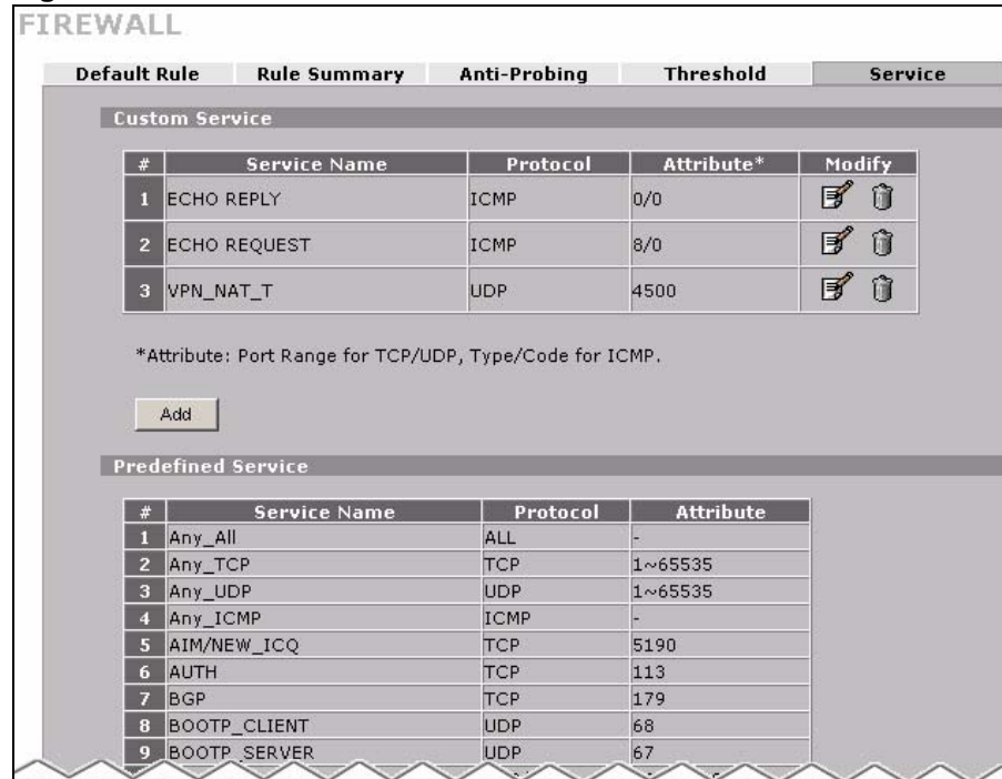
Figure 151 SECURITY > FIREWALL > Service
