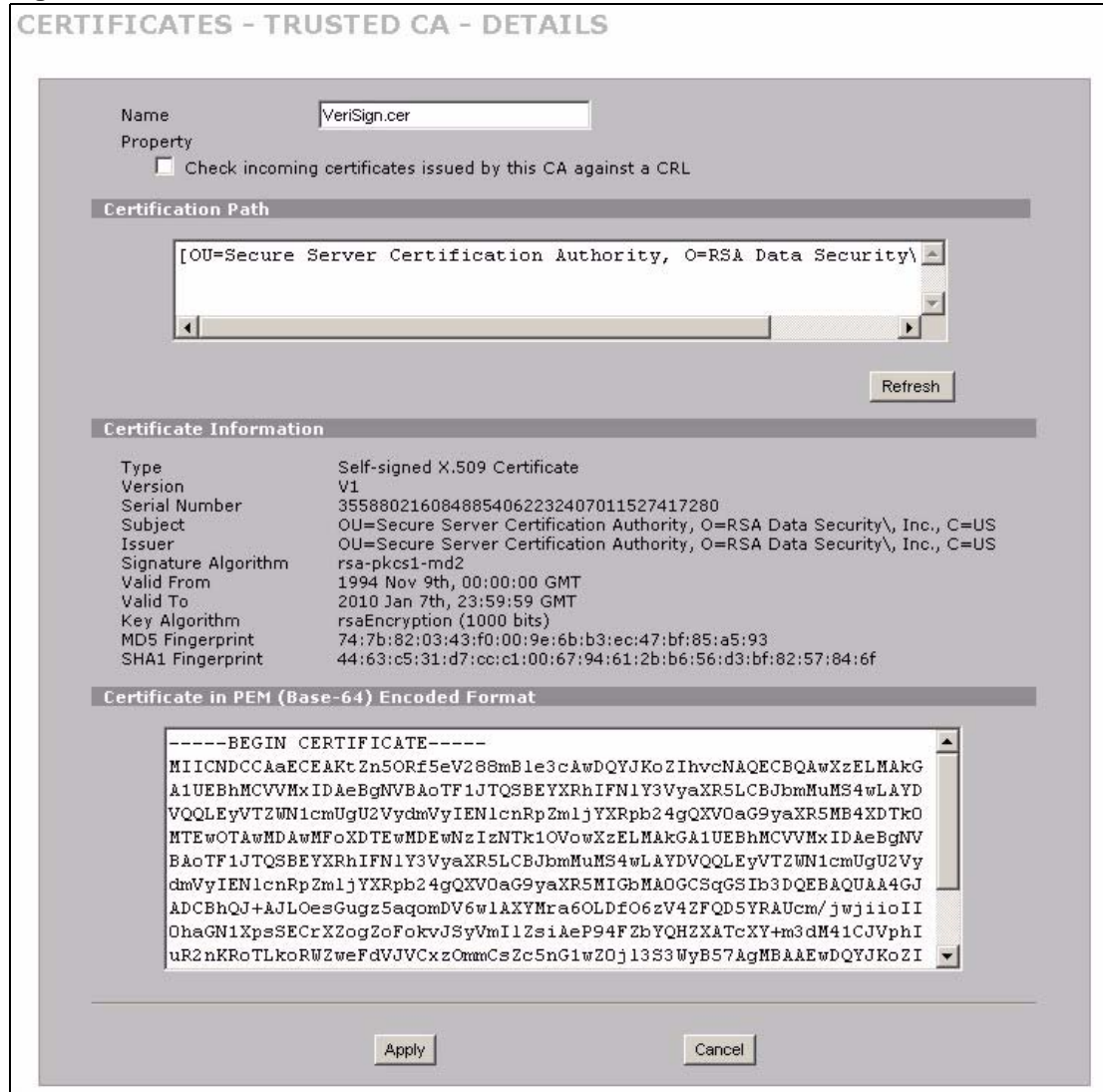
Figure 242 SECURITY > CERTIFICATES > Trusted CAs > Details
