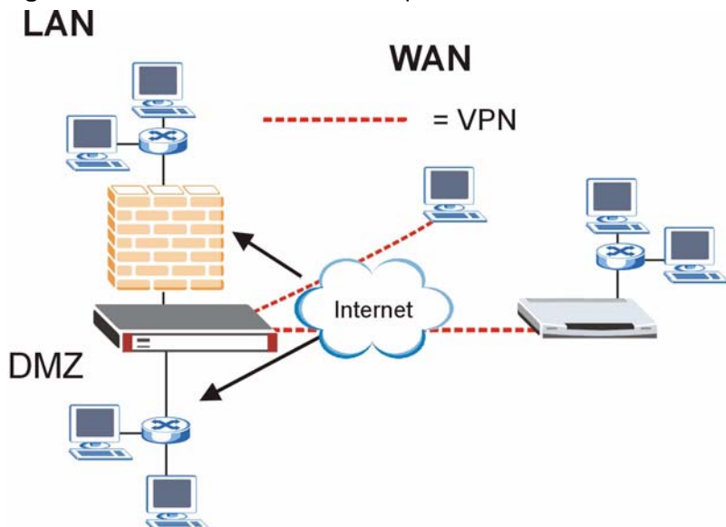
Figure 160 From VPN to LAN Example
