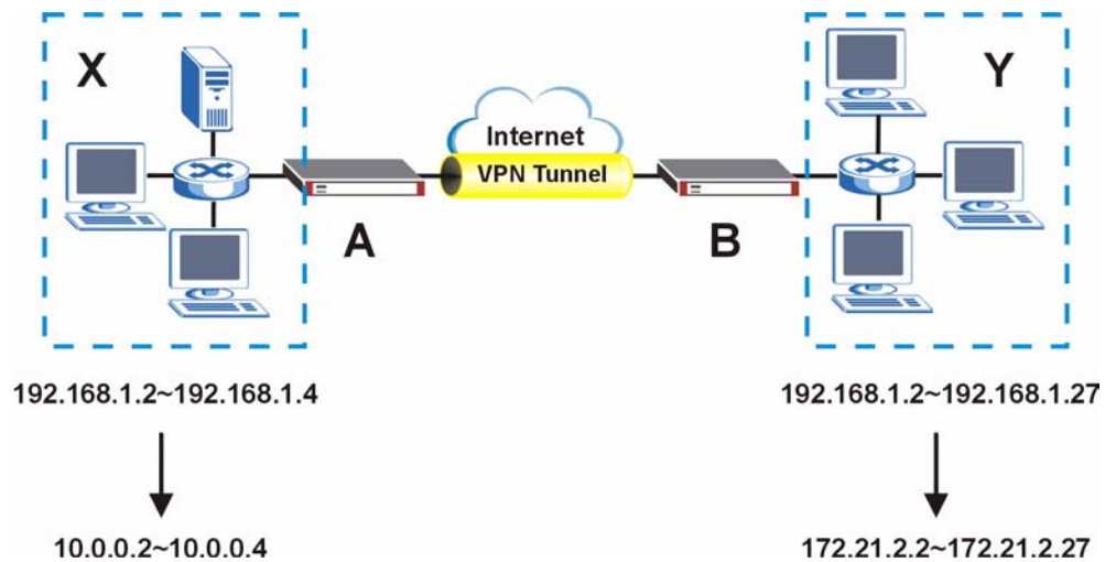
Figure 229 Virtual Mapping of Local and Remote Network IP Addresses
