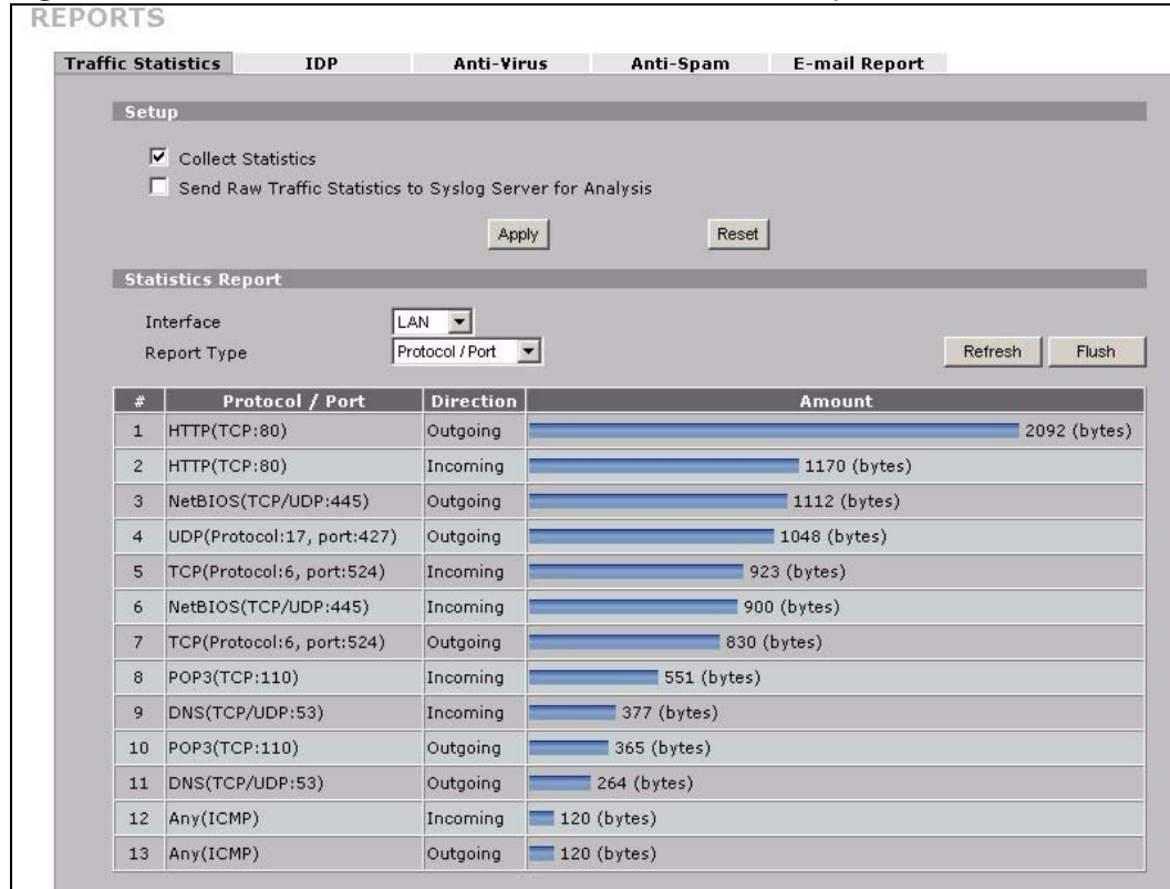
Figure 325 REPORTS > Traffic Statistics: Protocol/Port Example
